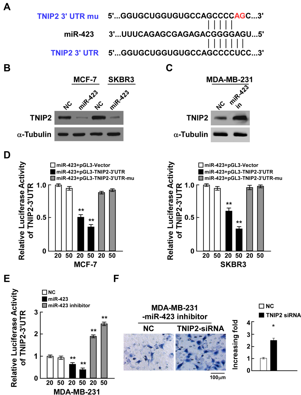
Figure 3 miR-423 directly targets TNIP2 in breast cancer cells. (A) Sequence of the TNIP2 3'-UTR shows the miR-423 binding seed region and mutation of the TNIP2 3'-UTR seed region. (B) TNIP2 protein expression in MCF-7 and SKBR3 cells transfected with miR-423 or negative control (NC). \alpha -Tubulin was used as loading control. (C) TNIP2 protein expression in MDA-MB231 cells transfected with miR-423 inhibitor or negative control (NC). (D) Relative luciferase activity of MCF-7 and SKBR3 cells co-transfected with increasing amounts of miR-423 mimic oligonucleotides (20 and 50 nM), and the pGL3 control reporter, pGL3-TNIP2-3'UTR reporter, or pGL3-TNIP2-3'UTR-mu reporter. (E) Relative luciferase activity of MDA-MB-231 cells transfected with increasing amounts of miR-423 mimic oligonucleotides (20 and 50 nM) or miR-423 inhibitor oligonucleotides (20 and 50 nM). (F) Transwell assay of indicated cells. Bars represent the mean \pm SD of three independent experiments; ** P < 0.01 , * P < 0.05 .
