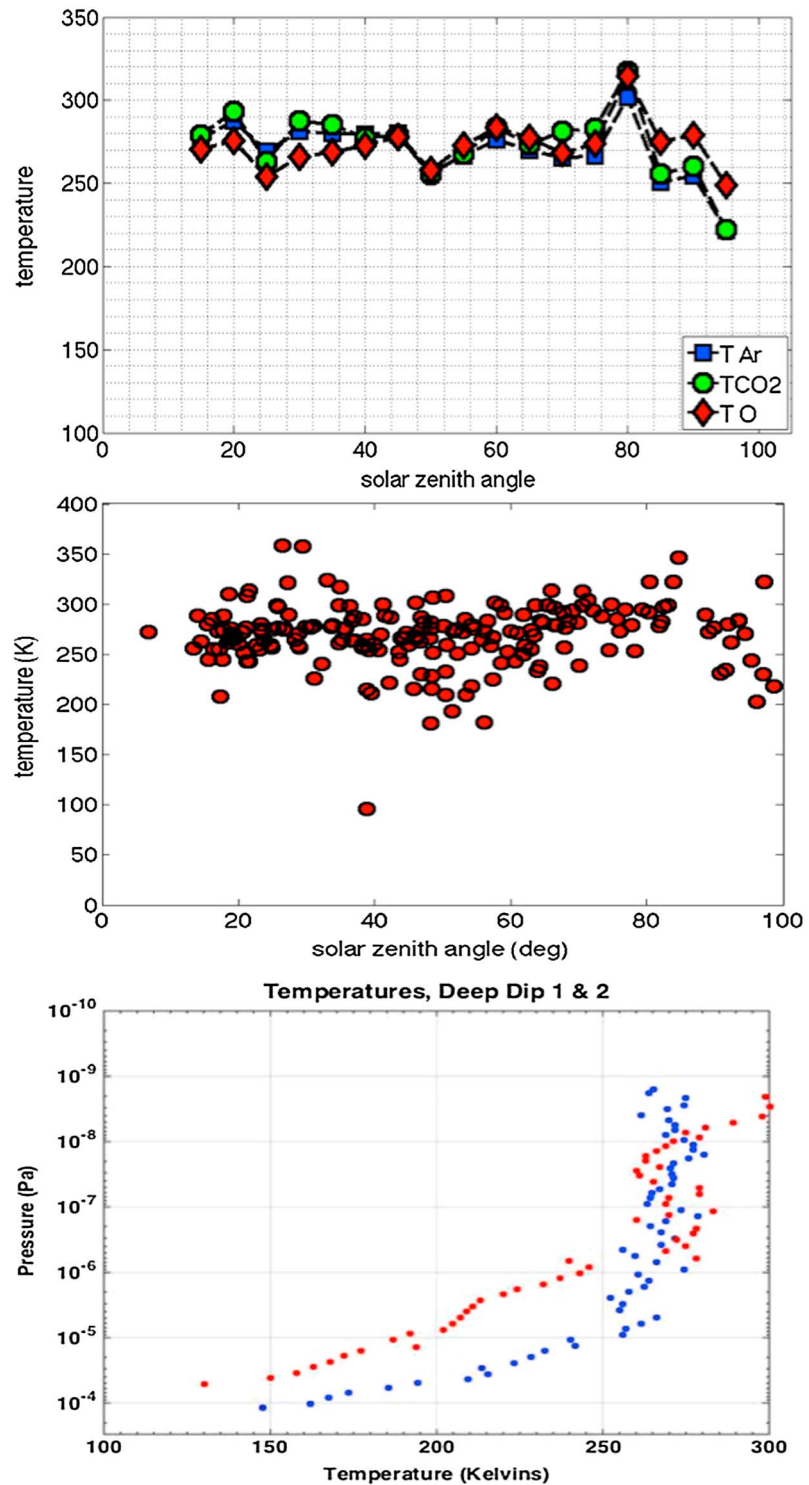
Figure 7. (top) Scale height temperatures derived from fits to NGIMS data between 200 and 300 km. Data are acquired in the Ls = 288–326 interval with latitude at periapsis 46° to –4.3°. (middle) The mean temperature in the 15–75° SZA region based on fitting inbound binned Ar, CO 2 , and O signals is 274 ± 6 K secured by averaging temperatures derived from these three independent determinations. The temperature drops by tens of Kelvin above 95° SZA. The apparent spike above SZA 85 may simply be a consequence of the limited sampling in these bins as illustrated in Figure S2. Temperature variation with (bottom) pressure for the two deep dip campaigns illustrate substantial differences at the lower altitudes and significant differences between the deep dip campaigns. The first deep dip (red) is centered around Ls = 289 at 46°N and the second (blue) around Ls = 326 near midlatitude. The Mars/Sun distance for these two deep dips was 1.41 and 1.48 AU, respectively.
