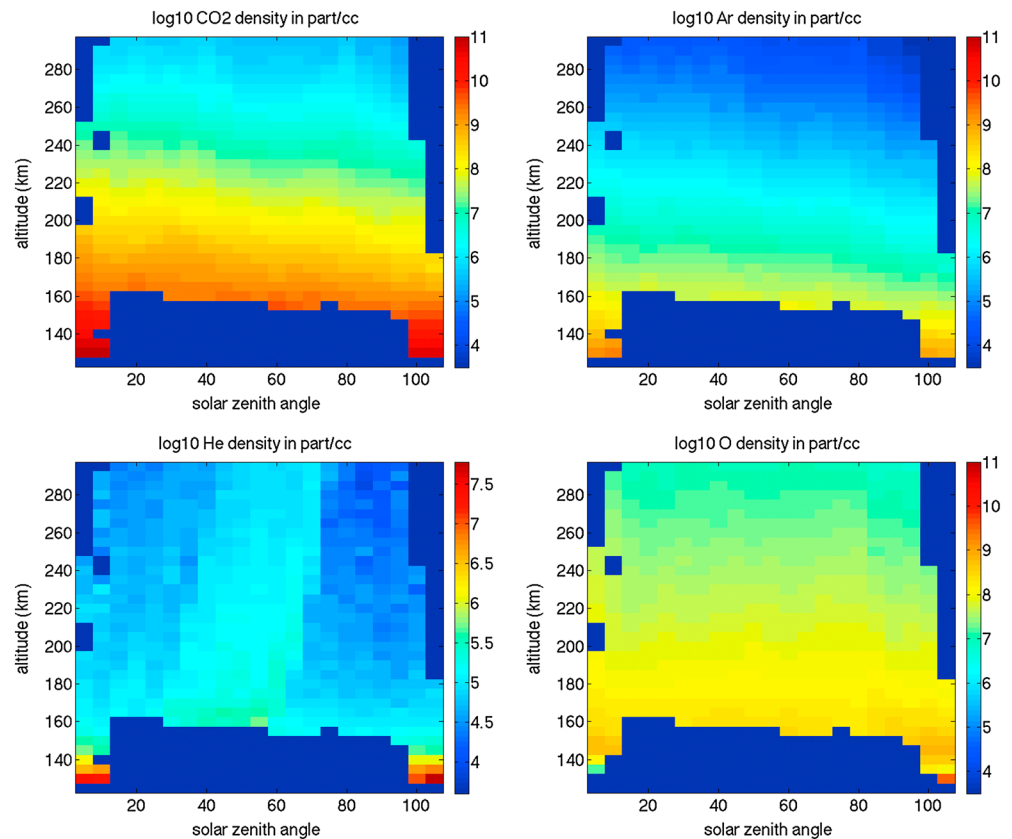
Figure 4. Variations of density for CO 2 , Ar, He, and O (Ls 288–326 and latitude at periapsis 46° to –4.3°) illustrates the gradual fall off of density at any altitude with solar zenith angle for (top left) CO 2 and (top right) Ar, the enhancements and variation with altitude of (bottom left) He in the 30–60° SZA range, and the abundance at high altitudes of (bottom right) O. More observations will be required to see if the He enhancements at 34–65° SZA will persist as the number of measurements in each bin increases. The two deep dips are evident at low and high solar zenith angles. The space represented by the darkest blue was not sampled.
