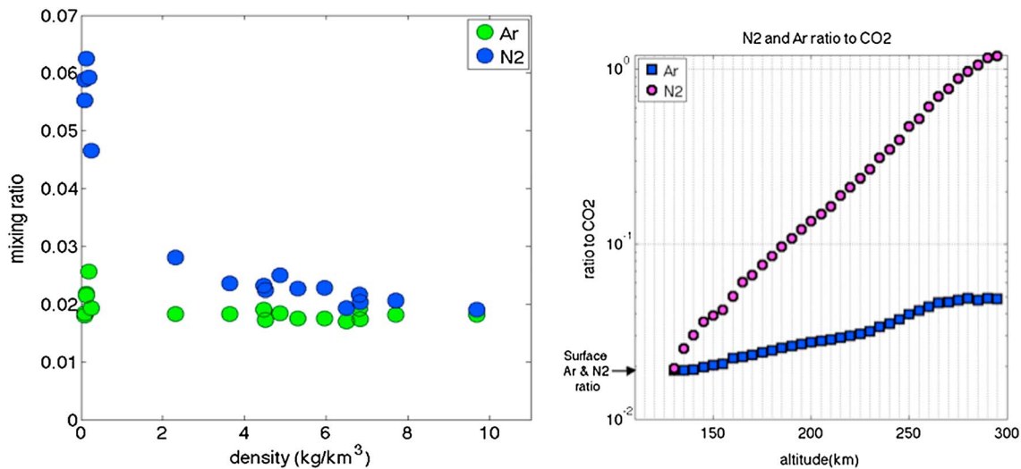
Figure 6. (left) 40 Ar and N 2 mixing ratios plotted versus total atmospheric density before, after, and during the second deep dip campaign (Ls = 326, latitude = –2° to –5°). Each point is the average density of either 40 Ar or N 2 at closest approach for that orbit. At the highest densities measured at about 10 kg/km 3 the lowest altitudes reached are ~130 km. At these altitudes the mixing ratios approach the bulk atmospheric mixing ratios established by the SAM experiment on the Curiosity rover. (right) The ratio of 40 Ar and N 2 to CO 2 are shown for 5° binned solar zenith angles less than 20°. These orbits include the second deep dip campaign and adjacent orbits where the higher altitudes are covered. These comparisons with surface mixing ratios demonstrate that the homopause for these three gases should be reached under these conditions at ~130 km.
