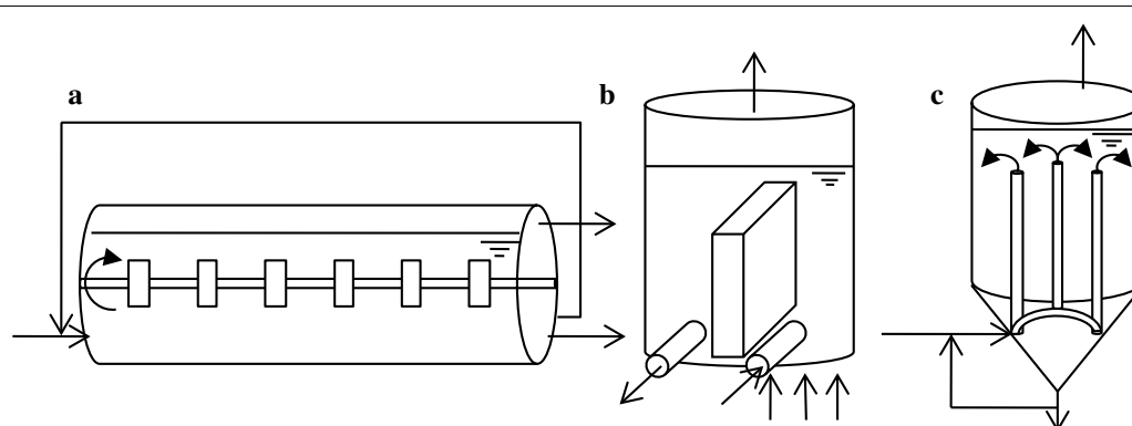
Fig. 3 Plug flow digesters for biogas production. a "Kompogas" reactor. Horizontal plug flow reactor. Additional mixing by axial mixer. Increased process condition stability by partial effluent recycling. Gas outlet on top of the outlet side. 23–28% total solids. b Valorga reactor. Substrate entry at the bottom; plug flow over a vertical barrier to the outlet. Additional mixing by biogas injection at the bottom. 25–35% total solid content. c Dranco reactor. Substrate entry with partial effluent recycling at the bottom, upward flow through substrate pipes. Downward plug flow to outlet. 30–40% total solids (Li et al. 2011; Nizami and Murphy 2010)
