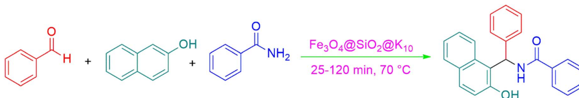
Scheme 2 Reaction of \beta -naphthol, benzaldehyde and benzamide catalyzed by \text{Fe}_3\text{O}_4@\text{SiO}_2@\text{K}_{10} .
