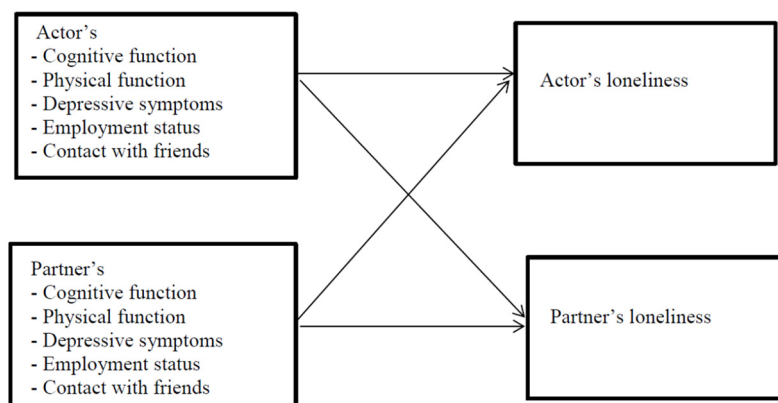
Figure 1. Actor-Partner Interdependence Model.
