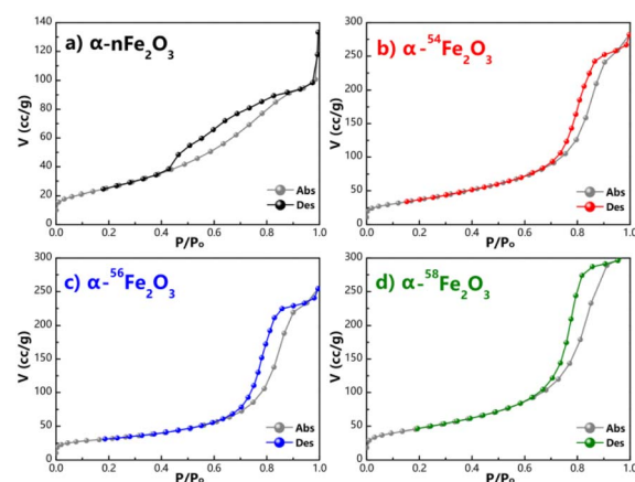
Fig. 2 Adsorption and desorption isotherms of N 2 of (a) \alpha - n Fe 2 O 3 , (b) \alpha - 54 Fe 2 O 3 , (c) \alpha - 56 Fe 2 O 3 , and (d) \alpha - 58 Fe 2 O 3 .
