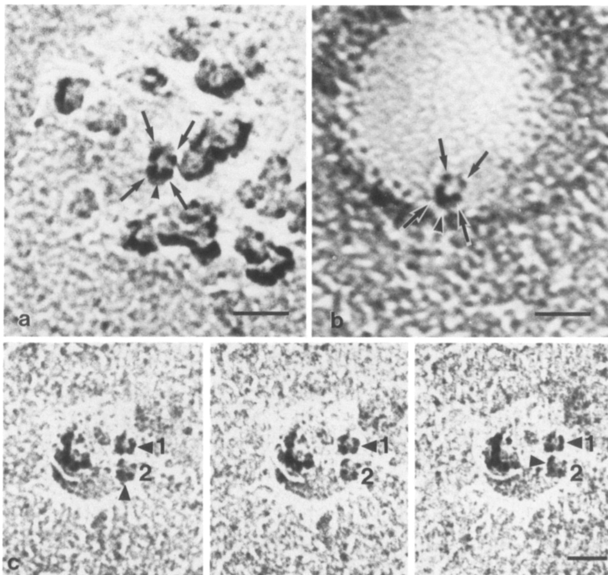
Figure 3. Rotary shadowing freeze-fracture of N -lauroylsarcosine stripped vesicles (a), CHIP28-incorporated proteoliposome (b), and liposome reconstituted with CHIP28 viewed at three different angles of observation, left to right by tilting the specimen on the microscope stage of -5^{\circ} , 0^{\circ} , and 10^{\circ} , respectively (c). CHIP28 IMPs are tetramers of \sim 8.5 -nm diam. Arrows show IMP subunits. The subunits are sometimes connected by a dense bridge (arrowheads). While the tetrameric structure is visible in IMPs 1 and 2 at all angles of observation, the relationship between subunits appears variable. Bars, 15 nm.
