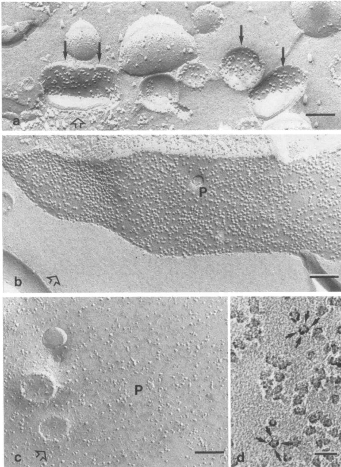
Figure 6. Freeze-fracture of intracellular membranes of CHIP28k-transfected CHO cells ( a ), CHIP28k-transfected cell plasma membrane P-face ( b ), and mock-transfected CHO cells plasma membrane P-face ( c ). Intracellular membranes ( full arrows ) and plasma membranes of CHIP28k-transfected cells contain additional large IMPs ( P , P-face). Empty arrows show direction of platinum shadowing. ( d ) Rotary shadowing freeze-fracture of the CHIP28k-transfected CHO cell plasma membrane P-face demonstrates the presence of tetramers ( arrows ). Bars: ( a-c ) 100 nm; and ( d ) 20 nm.
