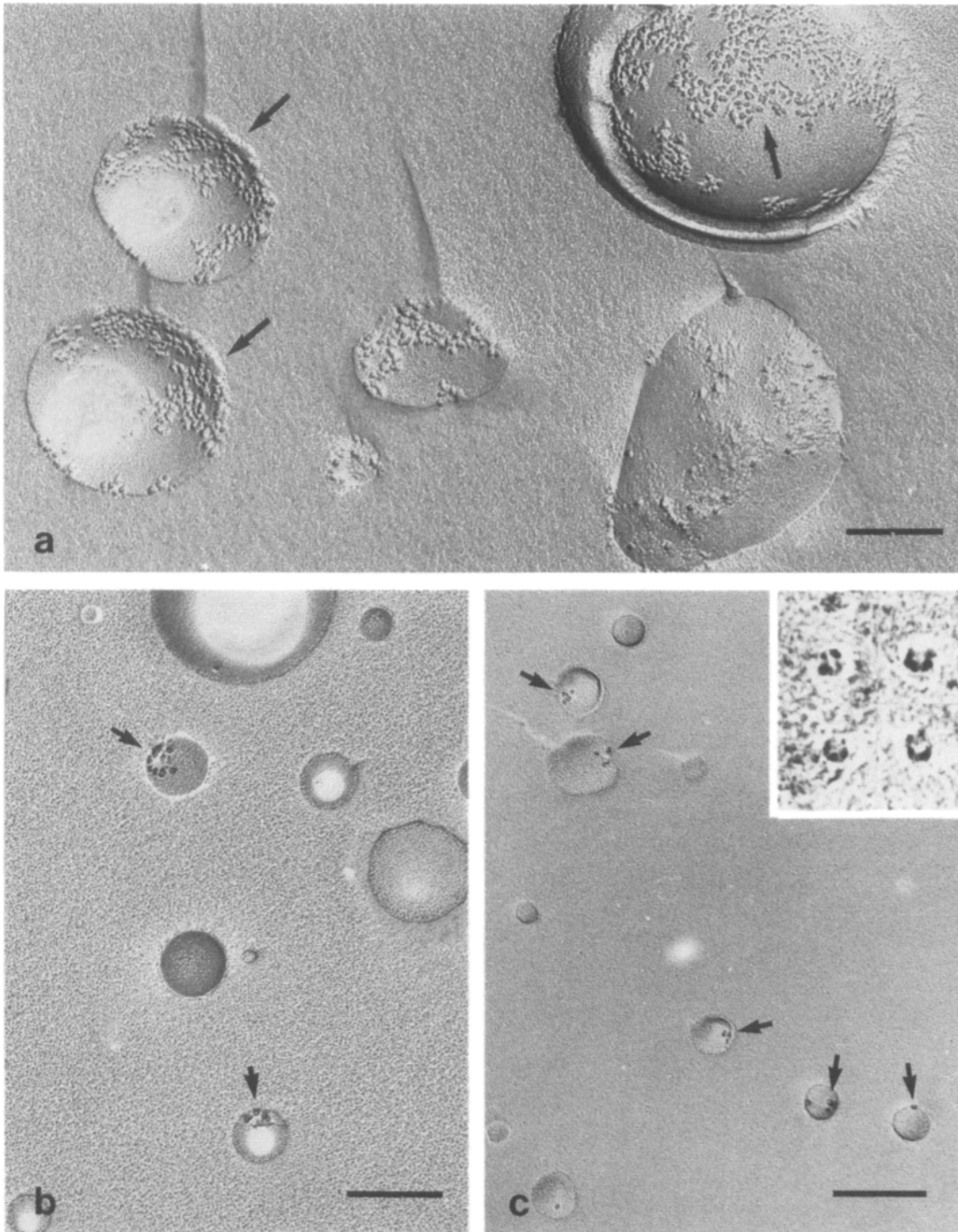
Figure 2. Freeze-fracture of KI-stripped erythrocyte membranes ( a ), N -lauroylsarcosine stripped vesicles ( b ), and CHIP28-incorporated proteoliposomes ( c ). Arrows show vesicles containing IMPs. ( Inset ) Gallery of four rotary-shadowed IMPs from CHIP28-incorporated liposomes ( \times 500,000 ). Note the tetragonal shape of the IMPs. Bars, 150 nm.
