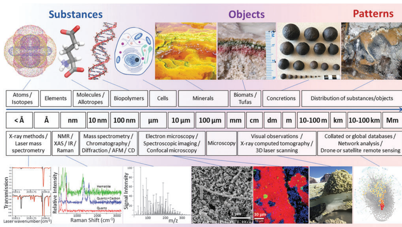
FIG. 2. Biosignatures and life detection methods range from microscopic (left) to planetary scales (right). A nested astrobiological approach will provide context for the physicochemical parameters and processes governing the preservation of biosignatures. Images created by R.J.G. using VMD software (Humphrey et al. , 1996). Top row images: carbonate formation in Río Tinto (Fernández-Remolar et al. , 2012); biomats (Des Marais, 2003); concretions (M.A.C.); and bio-vermiculation patterns, Cueva de Villa Luz, Tabasco, Mexico (P.J.B.). Life detection analytical techniques in bottom row (left to right) are laser spectroscopy (modified with permission from Leshin et al. , 2013); Raman spectra from 3.49 Ga Dresser Formation chert (D.M.B.); high-resolution mass spectrometry (Parker et al. , 2016); scanning electron microscopy (Chivian et al. , 2008); Raman spectra map (D.M.B.), photograph of sulfur deposits on the Borup Fiord Pass glacier (Lau et al. , 2017) computational network analysis ( http://dti.carnegiescience.edu ) (Morrison et al. , 2017).
