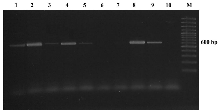
Fig. 2: Ethidium bromide stained 2% agarose gel of PCR products of Blastocystis sp. from pigs. M, molecular marker (100 bp); lanes 1, 2, 3, 4, 5 and 8, positive samples; lanes 6 and 7, negative samples; lane 9, positive control; lane 10, negative control
