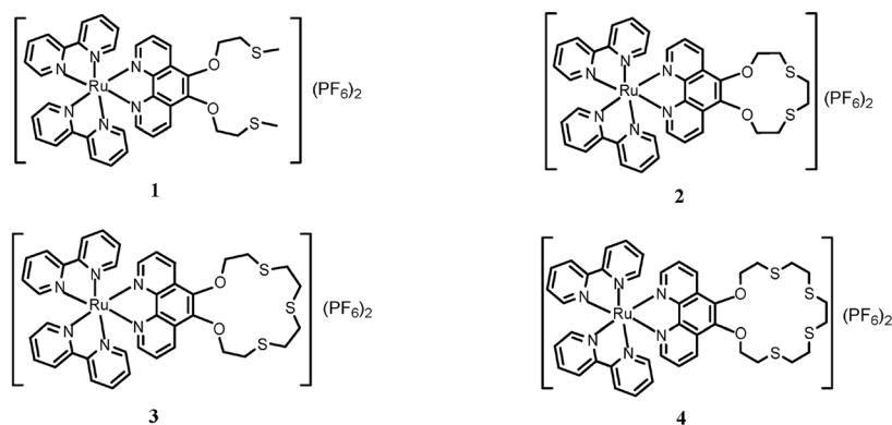
Scheme 1 Synthesis of ligands and complexes.
