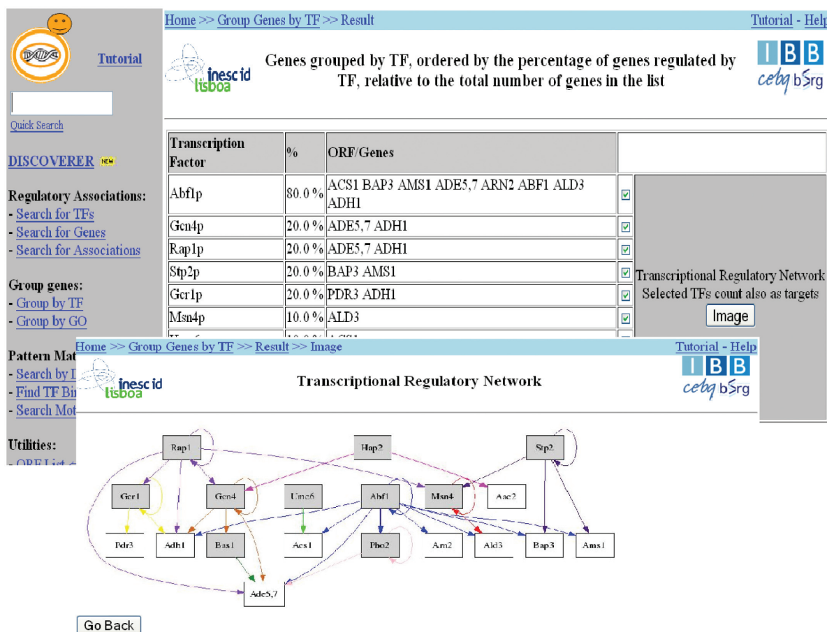
Figure 2. Sample pages showing the regulation graph obtained from the 'Group by TF' query. Shaded squares represent TF and white squares represent genes. Arrows represent interactions between each TF and target genes.
