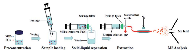
Fig. 1 Schematic illustration of MIPs-iEESI-MS for analysis of FQs.
