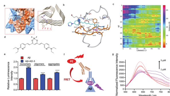
Fig. 3 Mechanism studies for epitope enhancers. (a) Molecule docking of the binding poses of CRANAD-17 with A \beta s (PDB: 5OQV). The protein surface is colored according to amino acid hydrophobicity (red: hydrophobic, blue: hydrophilic). The results suggest that CRANAD-17 binds to the hydrophobic moiety LVFF via the interaction of benzene and imidazole rings within the hydrophobic pocket of A \beta s. (b) A representative MD snapshot of CRANAD-17 binding with A \beta monomers. CRANAD-17 is highlighted in cyan, and all residues on A \beta that are within 5 Å of CRANAD-17 are shown in the stick representation. The residue loop 17–30 is highlighted in orange, and those that are within 5 Å of CRANAD-17 are also labelled. CA atoms on N and C termini are highlighted in marine and pink, respectively. (c) The distance map between each atom of CRANAD-17 and all heavy atoms in A \beta , y-axis is labelled as the peptide residue index. (d) The structure of CRANAD-3. (e) Quantitative data of dot blot assays for 1 μM A \beta 1–40 monomers, oligomers and aggregates with or without 2 μM of CRANAD-3 by using 4G8 antibody. CRANAD-3 could change the 4G8 antibody recognition and lead to increased readout for all A \beta species. (f) Illustration of the FRET assay. If CRANAD-3 could bind with the epitope of 4G8 antibody on A \beta monomers and form a ternary complex, the PE-labelled secondary antibody could serve as the donor molecule and excite CRANAD-3. (g) Fluorescence spectra of the mixture of A \beta monomers, 4G8 antibody and PE-labelled secondary antibody titrated with CRANAD-3 (1–3 μM). The typical FRET phenomenon is shown wherein the emission peaks of PE decreased while the emission peaks of CRANAD-3 simultaneously increased.
