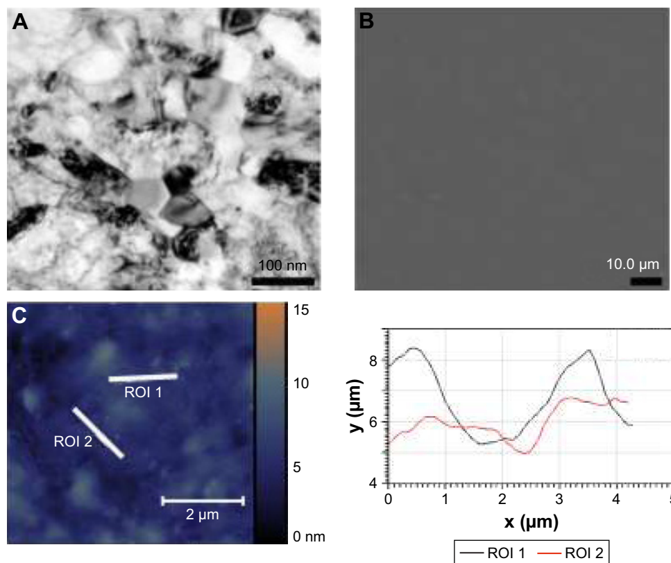
Figure 3 Characterization of the noncoated nanograined titanium samples. (A) Microphotograph of grain structure of nanotitanium samples. (B) Scanning electron microscopy of the polished titanium surface. (C) AFM reconstruction of the polished surface of nanotitanium with microtopography of the sample surface according to the AFM reconstruction.
