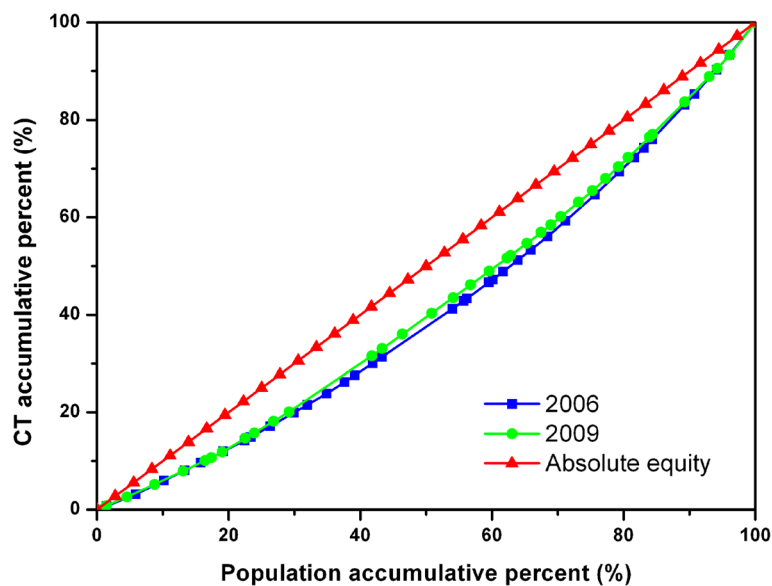
Figure 1 Lorenz Curve of CTs in all sample cities.
