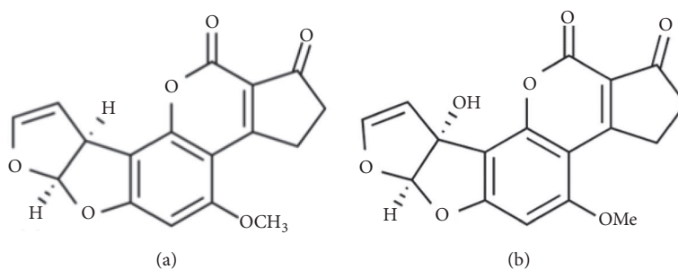
FIGURE 1: Chemical structure of AFB1 and AFM1. (a) Structure of AFB1. (b) Structure of AFM1.
