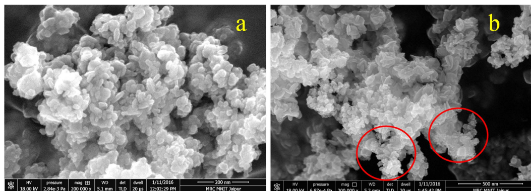
Figure 4. FESEM image of (a) CuS stacked plates and (b) CuS-Au-3 on CuS surface. Encircled area shows attachment of small particles on CuS plates.
