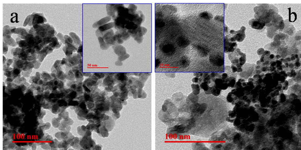
Figure 5. Low magnification TEM image of CuS (a) and CuS-Au-3 (b). Inset shows high magnification images of very small plates of CuS and very small particles of Au on CuS surface.
