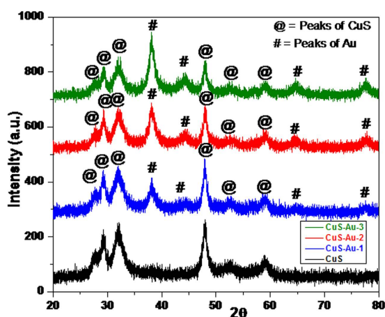
Figure 2. PXRD pattern of CuS and CuS-Au- n ( n = 1, 2, 3 ) showing the variation in the intensities of the highest intense peak of CuS and Au.
