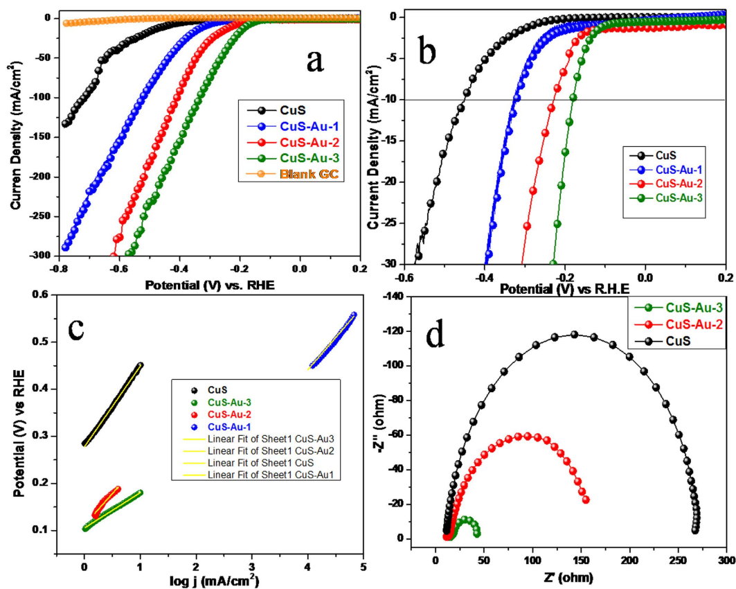
Figure 7. (a,b) Polarization curves for bare GC, CuS, CuS-Au-1, CuS-Au-2 and CuS-Au-3 in 0.5 M \text{H}_2\text{SO}_4 . (c) Tafel plots of CuS, CuS-Au-1, CuS-Au-2, and CuS-Au-3, (d) Nyquist plot of CuS, CuS-Au-2 and CuS-Au-3.
