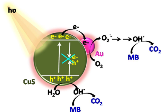
Figure 9. Schematic representation of MB degradation under visible light irradiation on CuS decorated with Au nanoparticles.
