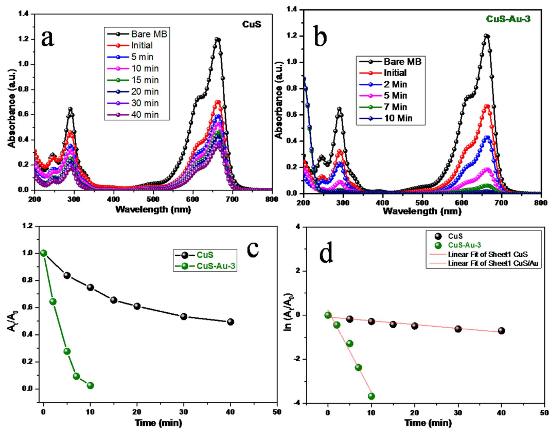
Figure 8. Photocatalytic decomposition of MB dye by using (a) CuS (b) CuS-Au-3 catalyst: absorbance vs. wavelength plot, (c) Plot of (A_t/A_0) vs. time for both CuS and CuS-Au-3, and (d) Plot of \ln(A_t/A_0) vs. time for both CuS and CuS-Au-3. Conditions: [MB] = 2 \times 10^{-5} M and catalyst = 10 mg.
