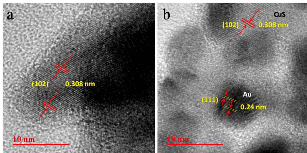
Figure 6. HRTEM image of (a) CuS and (b) CuS-Au-3.
