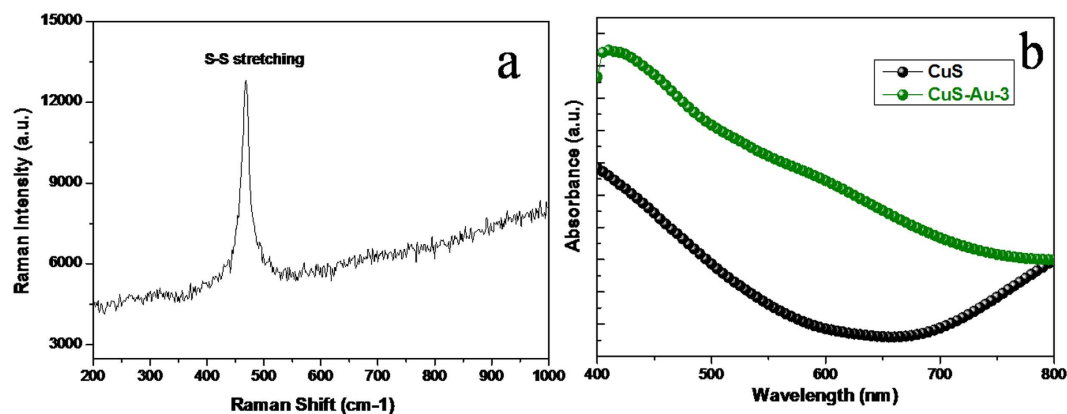
Figure 3. (a) Raman spectrum of CuS only and (b) UV-vis absorption spectrum of CuS and CuS-Au- n ( n = 3 only).
