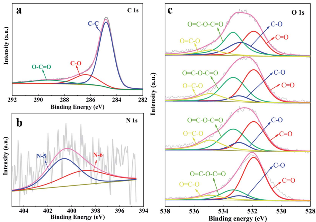
Fig. 5 XPS spectra of (a) C 1s; (b) N 1s for YPC-4; and (c) O 1s for the YPC-2, YPC-3, YPC-4, and YPC-5 samples.
