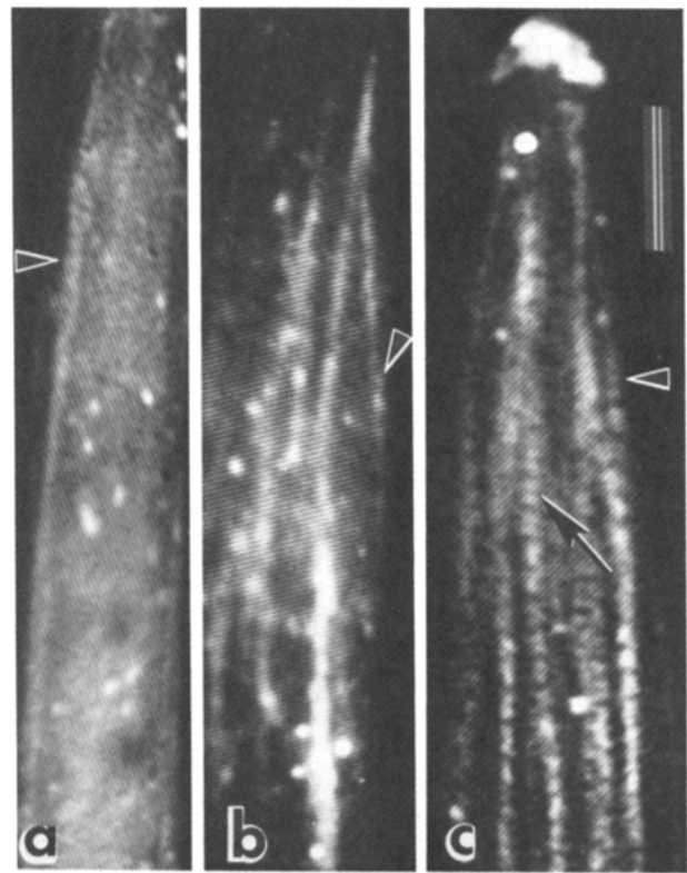
Figure 5. Living chick embryonic myotubes injected with IAR myosin light chains. ( a ) In myotubes injected on day 3 in culture, myosin light chains are incorporated in small periodic bands (arrowhead) in fibers near myotube membrane. There is also a high background of fluorescence in the cytoplasm and bright aggregates. ( b ) In myotubes injected on day 4 in culture there is a greater number of fibers containing periodic bands of fluorescence (arrowhead). Fluorescent aggregates and diffuse myotube fluorescence are also present in these myotubes. ( c ) In myotubes injected on day 5 in culture, most of the fluorescence is present in periodic bands of \sim 1.6 \mu m. In c spatial filtration (see Materials and Methods) was carried out on a previously summed image. The doublet composition of the fluorescent bands is seen more easily in this sharpened image (arrow in c ). An arrowhead in c points to a region of one fiber where small bands of fluorescence similar to those seen in younger myotubes ( a and b ) are visible. A concentration of myosin fluorescence is apparent in the ruffle at the end of the myotube. Bar, 10 \mu m.
