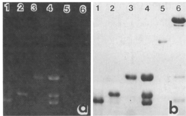
Figure 1. SDS-PAGE (12% acrylamide) of the IAR-labeled myosin light chains. (a) Fluorescence of the separated labeled light chains, LC-1, LC-2, and LC-3 in lanes 1, 2, and 3, respectively, and the total labeled light chain fraction in lane 4. (b) Coomassie Blue staining of the gel in a shows the labeled light chains in lanes 1–4, unlabeled G-actin standard in lane 5, and unlabeled myosin S-1 fraction in lane 6. The S-1 was prepared by chymotrypsin digestion, which degrades LC-2 (24), but not LC-1 and LC-3, as can be seen in lane 6.
