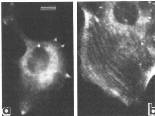
Figure 7. Two PtK 2 cells that were injected with IAR light chains and 5 h later exposed to 10% DMSO, a disrupter of stress fibers. (a) After 60 min in DMSO, myosin light chain fluorescence can be seen in aggregates in the cytoplasm but is absent from the nucleus. (b) 60 min after removal of DMSO myosin light chain fluorescence is found in a banded pattern in the reformed stress fibers. Bar, 10 µm.
