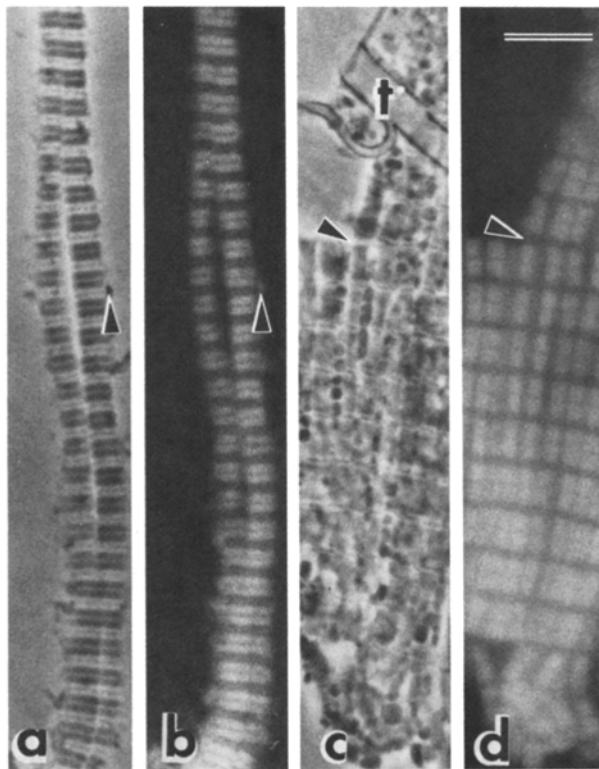
Figure 2. Isolated myofibrils attached to coverslips and exposed to the IAR-labeled mixed light chain fraction. (a and b) Phase and fluorescence of rabbit psoas myofibrils. Arrowheads point to a dirt speck adjacent to one of the Z bands. (c and d) Phase and fluorescence of myofibrils of insect flight muscle. Arrowheads point to a row of Z bands. A tracheid (t) visible in the phase does not bind the fluorescent light chains. In both types of muscle there is a doublet staining pattern in the A band. The nonstaining band in the center of the A band appears to be wider in the rabbit myofibrils than in the insect. All micrographs are the same magnification in order to emphasize the different A band sizes in a vertebrate versus an invertebrate muscle (1.6 vs. 3.3 \mu\text{m} ). Bar, 10 \mu\text{m} .
