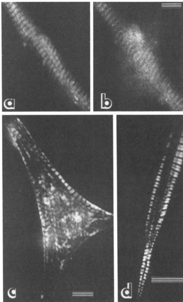
Figure 4. Living embryonic chick myotube co-injected with IAR light chains ( a ) and FITC- \alpha -actinin ( b ). Fluorescent bands show complimentary patterns of localization as expected from the A and Z band localization of the two proteins. Living embryonic cardiac myocytes injected with IAR myosin light chains ( c and d ). At higher magnification ( d ) A band doublet incorporation is clearly discernable. Bars, 10 \mu m.
