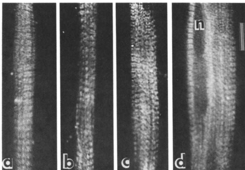
Figure 3. Living embryonic chick myotubes injected with IAR light chains after 7 d in culture. (a) Mixture of all three light chains; (b) LC-1; (c) LC-2; and (d) LC-3. In each case, the light chains are incorporated along the full length of the A band, with the exception of the center, where cross-bridges are absent. Spontaneous contractions were observed in many of the injected myotubes. No label was found in the nuclei (n in d). Bar, 10 \mu\text{m} .
