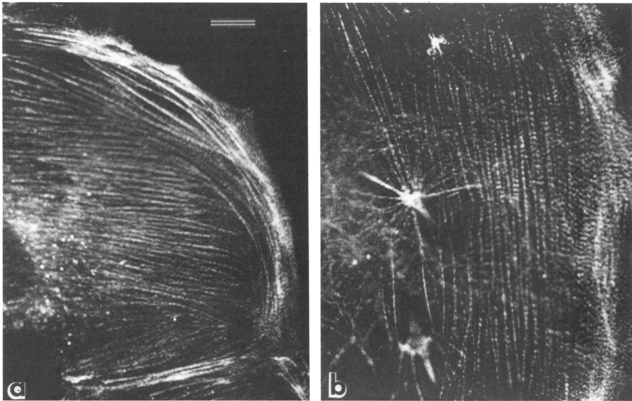
Figure 6. Living nonmuscle cells injected with fluorescent light chains. (a) PtK 2 cell showing striated pattern of myosin localization along the stress fibers. (b) Gerbil fibroma cell in which periodicity of myosin light chain fluorescence can be seen to be longer than in the epithelial PtK 2 shown at the same magnification in a . Bar, 10 µm.
