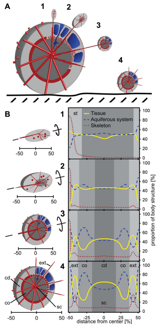
Figure 6 Scheme of bud development in T. wilhelma . (A) Four bud stages are characteristic, with the first three connected to the mother sponge by a stalk: Skeletal elements in red (megasclere bundles and aster spheres); megasclere bundles partly simplified as cylinders; Tissue in grey, separated into cortex (light grey) and choanoderm (dark grey). (B) Details of bud stages (left) and schematic graphs of morphological functional unit distribution. There are indications of rotational symmetry along the initial connecting stalk (st) in stages one to three (compare Additional file 4). Stage 4 buds display an adult-like body morphology with point symmetry to the skeleton centre (sc; see Additional file 5). Choanoderm development starts in stage 2, accompanied by the development of the megaster spheres in stage 3. Differentiation into a cortex (co) and choanoderm (cd) is characterized by the development of the aquiferous system (larger canals in stage 2; lacunae in stage 3). Body extensions (ext) (filaments) are found in stage 4 buds. For further details see text.
