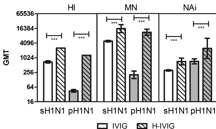
Figure 1 Serological characterization of pre-pandemic IVIG (open bars) and post-pandemic H-IVIG (hatched bars). Antibody titers against the seasonal H1N1 strain A/New Caledonia/20/1999 (sH1N1) (white bars) and pandemic A/California/07/2009 (pH1N1) (grey bars) were determined by hemagglutination inhibition (HI), microneutralization (MN) and enzyme-linked lectin assay (ELLA, reported as NA inhibition [NAi]), respectively. Results are given as geometric mean titer (GMT) \pm 95% confidence interval (CI). Statistical differences were calculated by unpaired Student t-test analysis (GraphPad Prism software). *** P < 0.0001 . GMTs were calculated by testing 13 individual lots of IVIG and 2 lots of H-IVIG.
