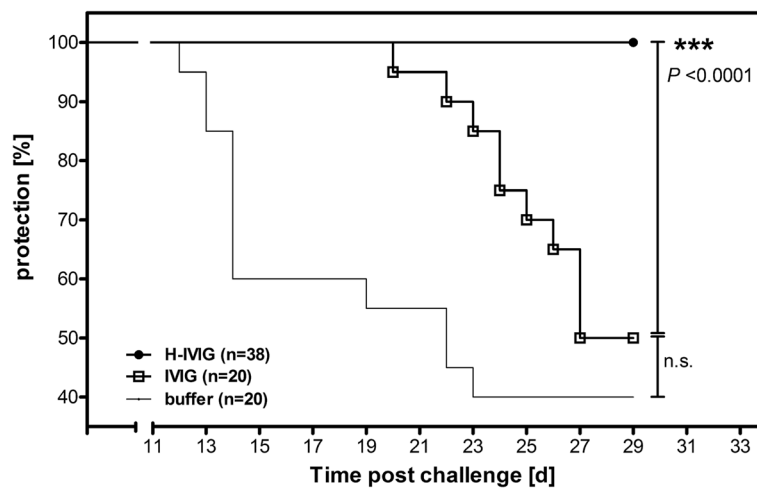
Figure 2 Protective efficacy of pre-pandemic IVIG and post-pandemic H-IVIG. To evaluate passive protection efficacy, SCID mice were intraperitoneally administered with 200 \mu l of pH1N1 hyperimmune IVIG (two lots, HI titer 1:1,280) or pre-pandemic IVIG (pool of five lots, HI titer 1:70) 3 days prior to challenge with 6 \times 10^4 TCID 50 of wild-type pH1N1 by intranasal instillation. The control group received 200 \mu l of PBS and survival was monitored for 29 days. Statistical differences between the IVIG group and the PBS control group, and between the IVIG group and the H-IVIG group, were calculated with a Log-rank (Mantel-Cox) test using the GraphPad Prism software. Abbreviations: d, days; n.s., not significant; IVIG, pre-pandemic intravenous immunoglobulin; H-IVIG, hyperimmune intravenous immunoglobulin.
