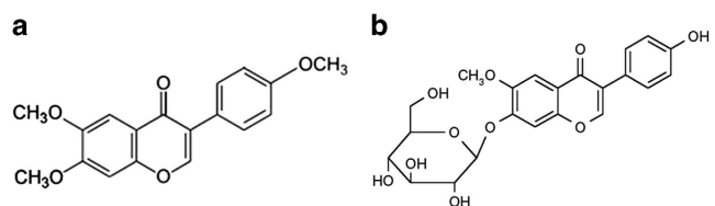
Figure 1 The chemical structure of TMF and glycitin. (a) TMF (4',6,7-trimethoxyisoflavone). (b) Glycitin (4'-hydroxy-6-methoxyisoflavone-7-D-glucoside). TMF, 4',6,7-trimethoxyisoflavone.
