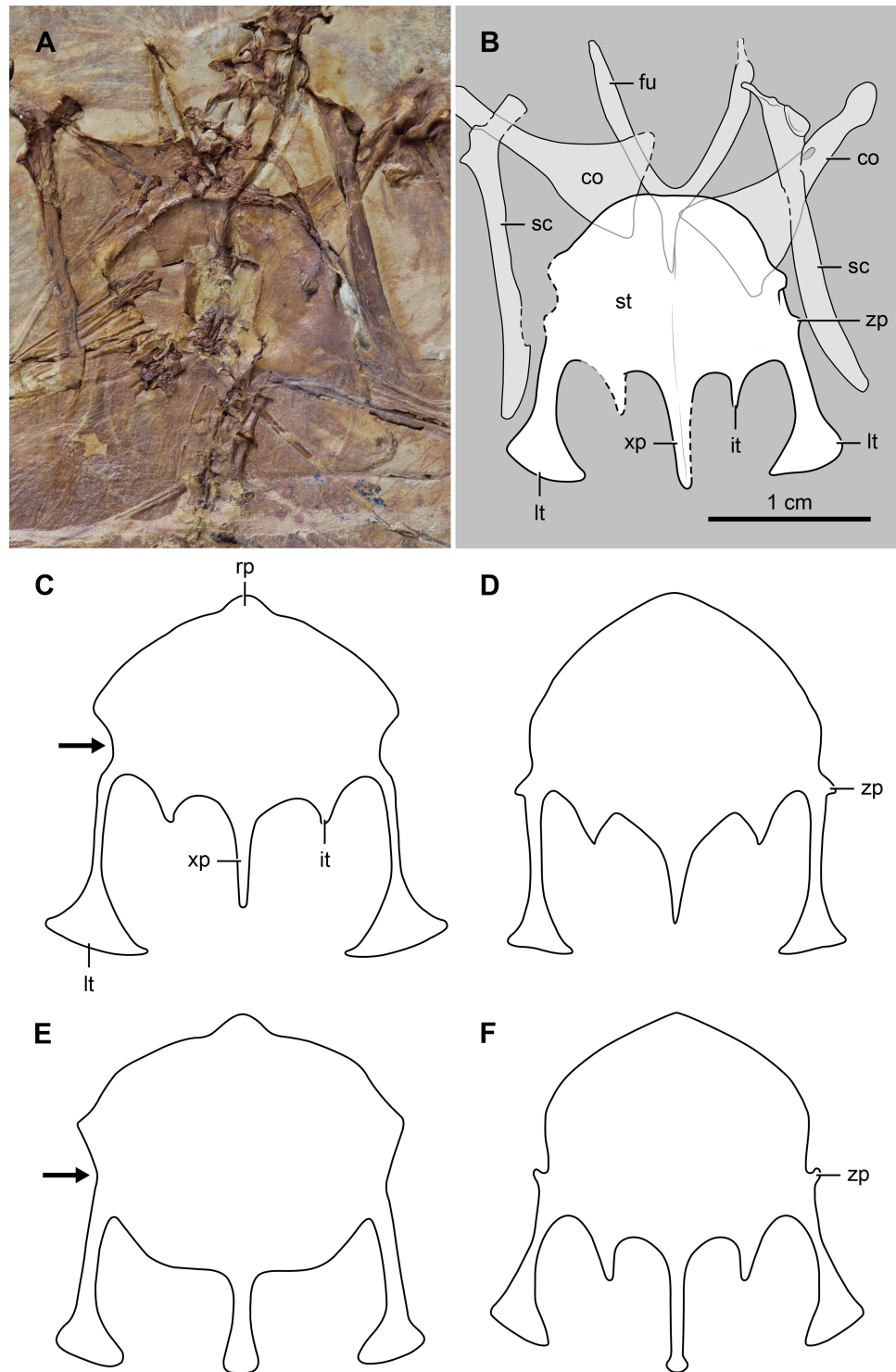
Fig 3. Comparison of the sterna of selected enantiornithines. (A, B), photograph and interpretative drawing of Junornis houi , BMNHC-PH919a; (C), Houornis caudatus ; (D), Cathayornis yandica (IVPP 9769); (E), Eocathayornis walkeri (IVPP 10916); (F), “ Cathayornis chabuensis ” (OFMB-3). Abbreviations: co, coracoid; fu, furcula; it, intermediate trabecula; lt, lateral trabecula; rp, rostral process; sc, scapula; st, sternum; xp, xiphoid process; zp, zyphoid process. The black arrow in C and E points at the concave costal margin of the sternum of Houornis caudatus and Eocathayornis walkeri . Drawings C-F are not to scale.
