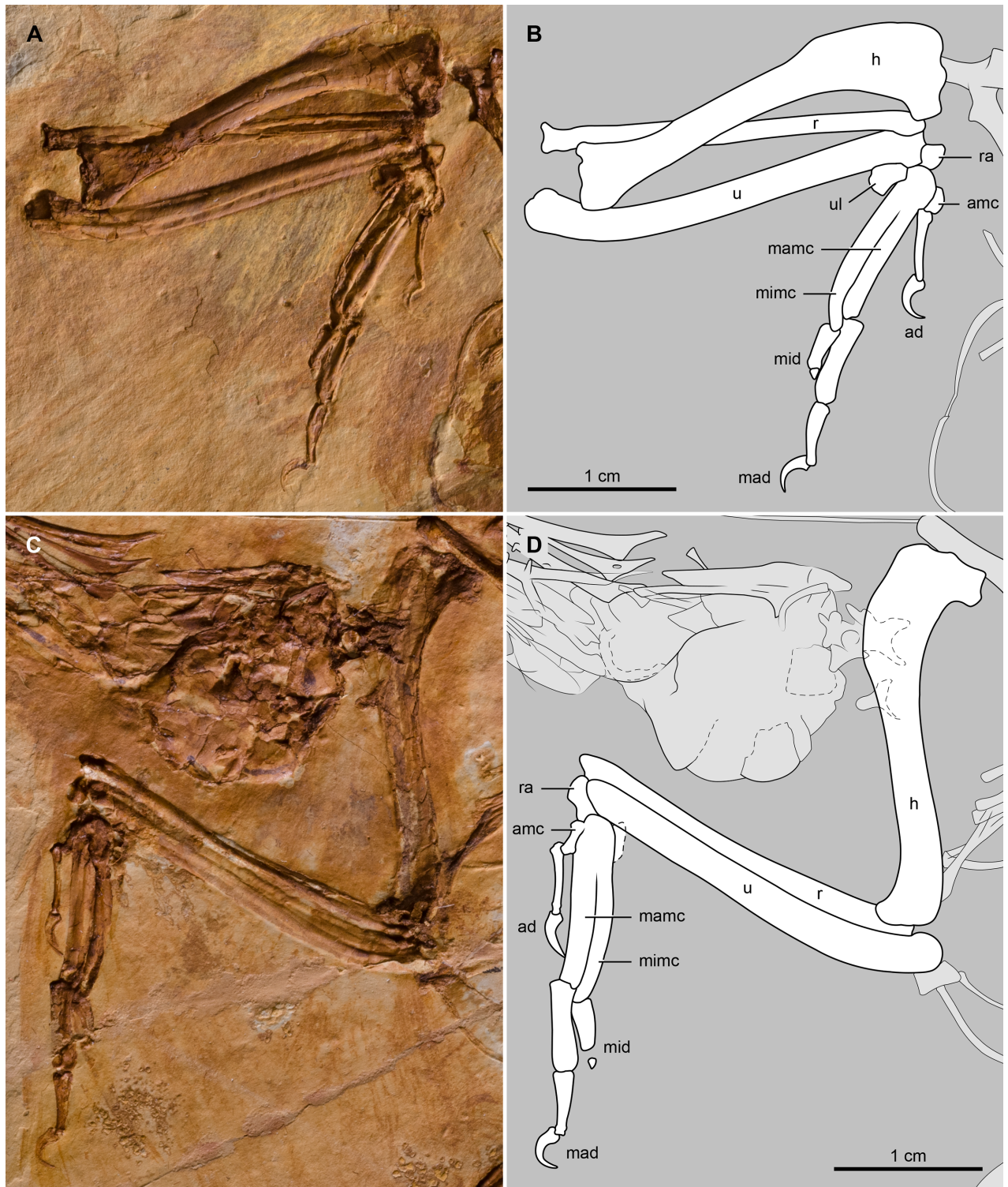
Fig 5. Photograph and interpretative drawing of the forelimb of Junornis houi . (A, B) BMNH-C-91919a and (C, D) BMNH-C-91919b. Abbreviations: ad, alular digit; amc, alular metacarpal; h, humerus; mad, major digit; mamc, major metacarpal; mid, minor digit; mimc, minor metacarpal; r, radius; ra, radiale; u, ulna; ul, ulnare.
