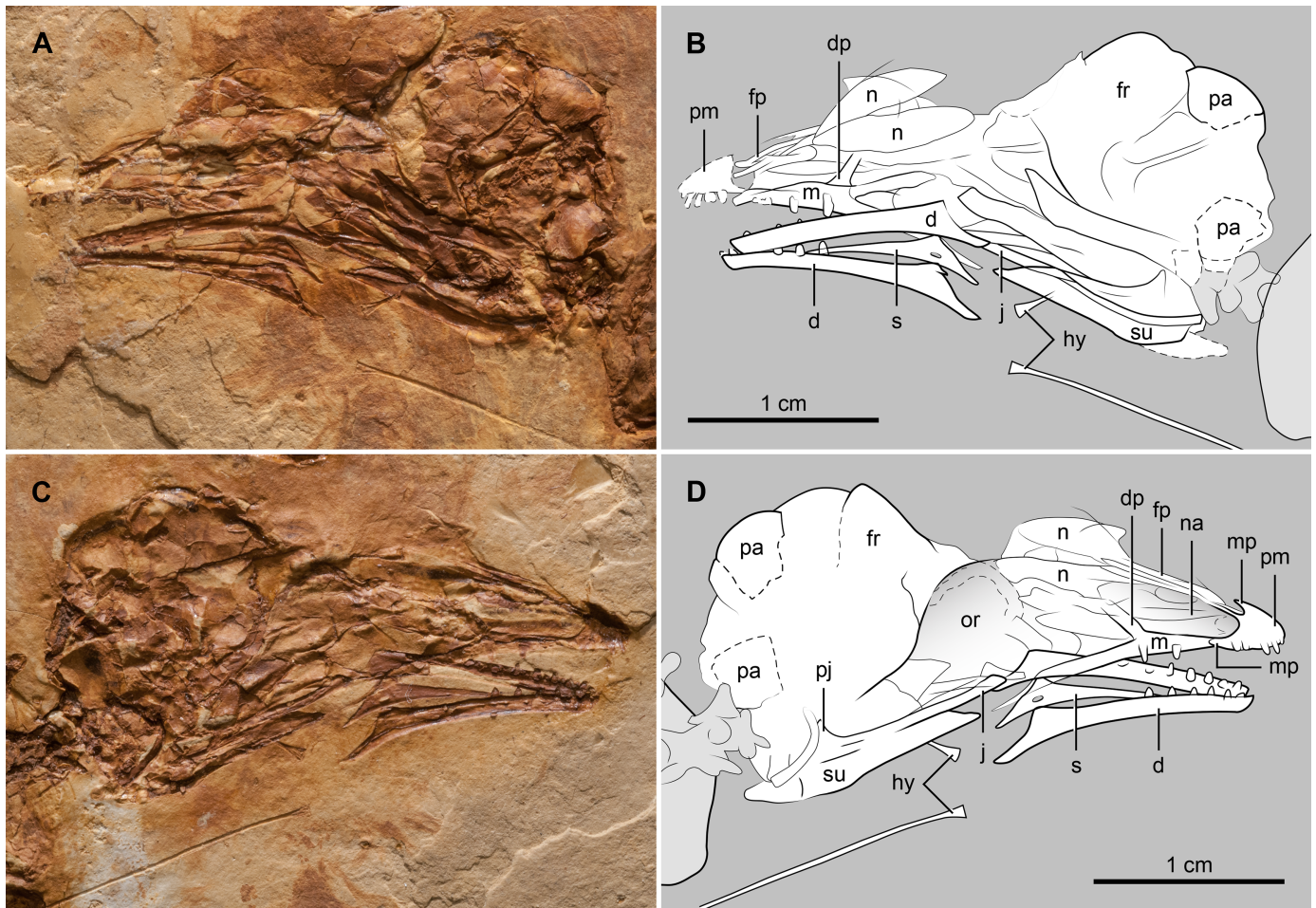
Fig 2. Photograph and interpretive drawing of the skull of Junornis houi . (A, B) BMNH-919a and (C-D) BMNH-919b. Abbreviations: d, dentary; dp, dorsal process of maxilla; fp, frontal process of premaxilla; fr, frontal; hy, hyoid; j, jugal; m, maxilla; mp, maxillary process of premaxilla; n, nasal; na, external nares; or, orbit; pa, parietal; pj, postorbital process of jugal; pm, premaxilla; s, splenial; su, surangular.
