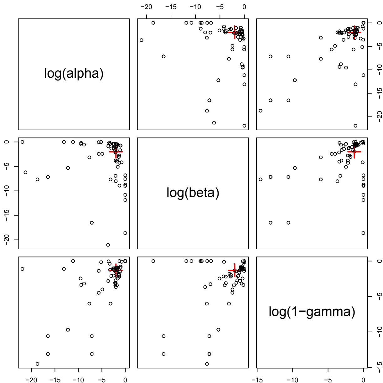
Figure 7 Optimum values of \alpha , \beta and 1 - \gamma . Pairwise plots of the optimum values ( \log_{10} ) of \alpha , \beta and 1 - \gamma . Each point represents the optimum values of \alpha , \beta and 1 - \gamma for one of the reference arrays. The crosses mark the positions of the actual values of \alpha , \beta and 1 - \gamma used in the analysis ( \alpha = 0.01 , \beta = 0.01 and 1 - \gamma = 0.05 ).
