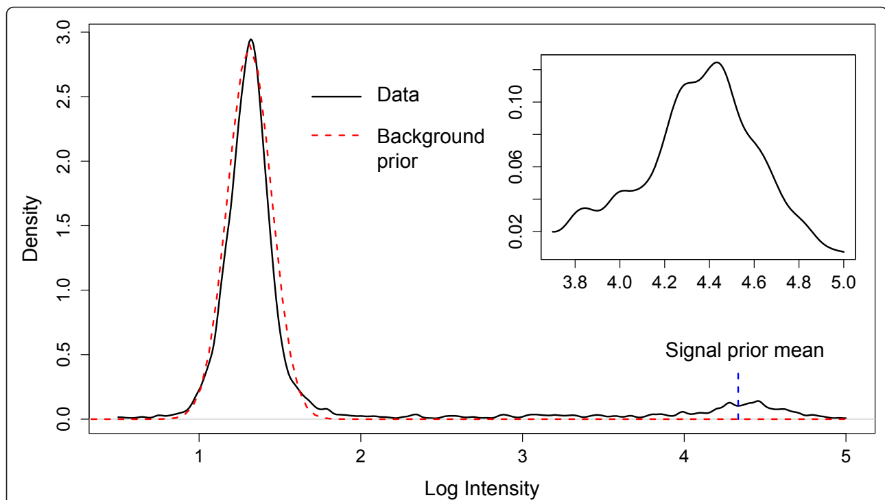
Figure 3 Density estimate of CPS probe intensities. Density estimate of the log probe intensities for 432 cps genes from a Streptococcus pneumoniae serotyping microarray testing strain 24A. The background prior distribution N(\mu_0, \sigma_0^2) and the value of the signal prior mean \mu_{(1)} for this data are also shown. The inset shows the signal part of the distribution in more detail.
