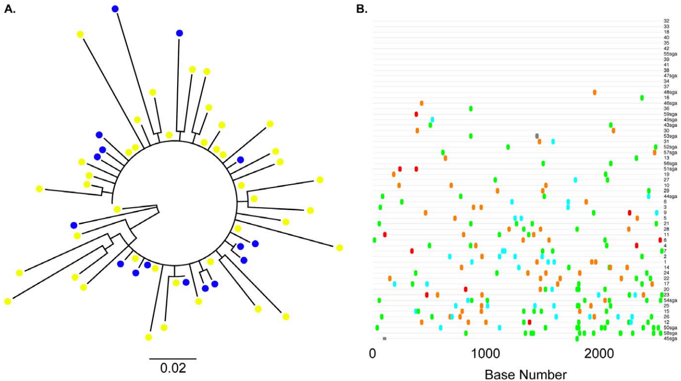
Figure 2. The relationship between SHIV-162P3 stock full-length env obtained by standard cloning and single genome amplification. (A) An unrooted maximum likelihood tree constructed with standard clones and 17 previously reported sequences generated by single genome amplification. Blue circles, SGA clones; Yellow circles; standard clones. The horizontal bar represents genetic distance. (B) Highlighter plot indicates the gp160 nucleotide variation between clones. Clones are numbered sequentially; SGA clones are depicted with “sga” after the clone number. Adenine, green; Cytosine, aqua; Thymine, red; Guanine, orange. Grey bars indicate missing sequence. doi:10.1371/journal.pone.0028047.g002
