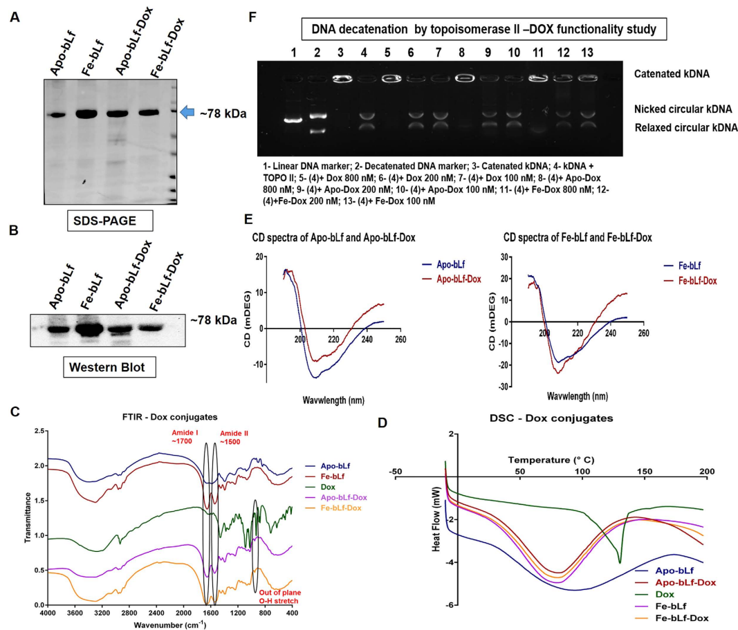
Figure 1. Synthesis and characterisation of bLf-Dox conjugates. (A) Image indicates the purity of synthesised forms of bLf-Dox conjugates prepared from Apo-bLf and Fe-bLf using SDS PAGE represented by a single non-denatured band around 78 kDa. (B) Western blot was carried out for the synthesised bLf-Dox conjugates against goat anti-bLf monoclonal antibody (1:1000) showing antigen reactivity ~78 kDa. (C) FTIR spectroscopy analysis was performed between 4000 and 400 \text{cm}^{-1} at a resolution of 4 \text{cm}^{-1} averaging 10 scans. The spectrum of each sample was then plotted with percentage transmittance against wavenumber. Crucial peaks are highlighted in the spectra. (D) The thermal stability and the crystallinity of the conjugates was studied using differential scanning calorimetry (DSC) and the endotherm has been represented. (E) The secondary structural characteristics of Apo-bLf and Fe-bLf before and after Dox conjugation was studied using Circular Dichroism (CD) spectroscopy. CD values were obtained for secondary structure prediction at a wavelength range of 250 nm to 190 nm at an interval rate of 0.1 nm/s and the resultant CD spectra of milli degrees vs wavelength was plotted in the graph. The functional stability of Dox in the form of conjugates was confirmed by its ability to inhibit human topoisomerase II (TOPO II) to decatenated human kinetochore DNA (kDNA). The presence of nicked circular kDNA and relaxed circular kDNA was considered as a positive for the activity of TOPO II uninhibited by Dox. The presence of only the catenated kDNA at the wells is considered complete inhibition of TOPO II by Dox.
