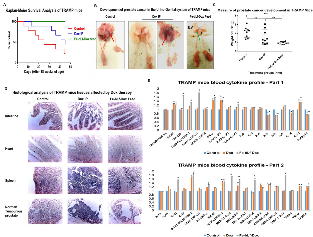
Figure 6. Fe-bLf-Dox conjugates inhibited tumour development and prolonged the survival of TRAMP mice. (A) Kaplan—Meier survival analysis of TRAMP mice groups (Control, Dox IP and Fe-bLf-Dox diets) for n = 9 mice per group following treatment post 18 weeks of age for 45 days. (B) Dissected Urino-Genital Tract (UGT) of the TRAMP mice displaying seminal vesicles (S.V), bladder (B), testes (T) and the prostate (Red = Tumourous; Green = Normal). (C) Normalised UGT weights against the mice body weights as a measure of tumour development in TRAMP mice in control, Dox IP and Fe-bLf-Dox feed groups ( n = 9 ). Two-way ANOVA was performed to evaluate statistical significance followed by post-hoc analysis by Tukey's test. (D) Histopathological analysis of TRAMP mice tissues post haematoxylin and eosin staining viewed under optical light microscope 400X magnifications. Sections of mice intestine, heart, spleen and prostate are provided. (E) Proteome profiler array analysis of serum cytokine expression profile of TRAMP mice treated with Dox and Fe-bLf-Dox ( n = 3 ). Image J analysis of micro-array profile was carried out and relative fold change in the integrated density of each cytokine has been represented as histogram (Mean \pm S.D.).
