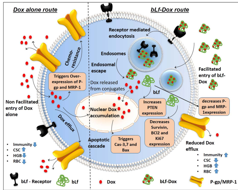
Figure 7. Schematic representation summarizing the inferences of this study about the role of Fe-bLF-Dox conjugates in overcoming drug resistance. Dox alone (Left) causes increase in chemo-resistance by up-regulating P-gp and MRP-1 expression thereby getting effluxed out of the cancer cells quickly causing minimal damage. bLf-Dox conjugates are easily internalised by cancer cells without triggering P-gp increase and facilitates longer nuclear retention of Dox increasing its cytotoxicity. Meanwhile bLf also decreases survivin, P-gp and MRP-1 expression and increases PTEN expression to decrease chemo-resistance and trigger cancer cell apoptosis. Fe-bLF-Dox treatment in TRAMP mice also reversed the RBC and HGB loss due to Dox treatments and induced anti-tumour immunogenicity. The schematic illustration was generated by modifying images purchased in the PPT Drawing Toolkits-BIOLOGY Bundle from Motifolio, Inc.
