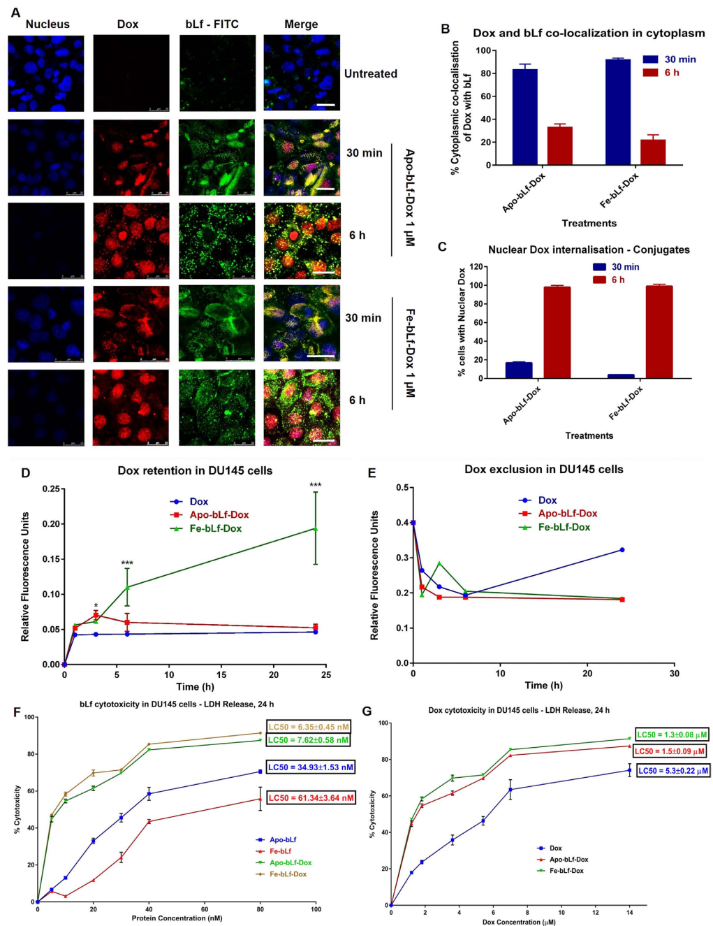
Figure 2. bLf-Dox conjugates promote greater retention of Dox resulting in enhanced cancer cytotoxicity.
