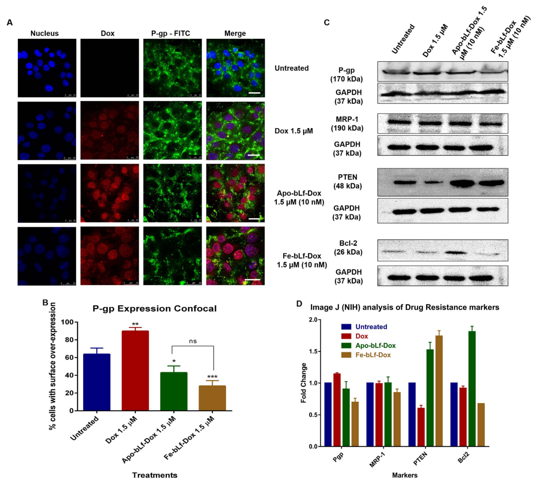
Figure 4. bLf-Dox conjugates are capable of overcoming molecular drug resistance pathway.
