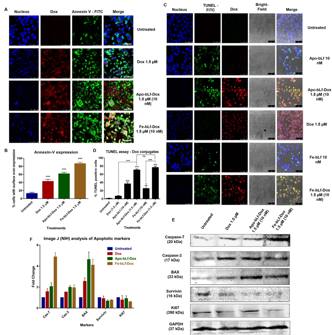
Figure 3. bLf-Dox conjugates treatment induces cancer cell apoptosis. (A) Representative confocal microscopy images of DU145 cells showing the expression of annexin-V as a marker of apoptosis post treatment with Dox, Apo-bLf-Dox and Fe-bLf-Dox. The annexin-V was stained using immunofluorescence with rabbit anti-annexin-V primary antibody and anti-rabbit-IgG FITC conjugated secondary antibody represented in green fluorescence. Dox auto-fluorescence is represented in red. The nucleus was counterstained with DAPI (blue). Scale bar = 50 µm. (B) Percentage of cellular annexin-V expression from 5 images each was calculated and represented as a histogram (Mean ± S.D.). (C) The presence of fragmented DNA as an end product of apoptotic cascade within the cell was considered as the confirmatory test for induction of apoptosis especially the Dox mediated DNA damage using TUNEL assay. The nucleus was counterstained with DAPI and Dox auto-fluorescence is represented in red. (D) Percentage of TUNEL positive cells from 5 images each has been represented as a histogram. Statistical analysis was performed using one-way ANOVA and a post-hoc Tukey's test. (E) The molecular regulation of apoptosis was studied using Western blots for various apoptotic markers. The Western blotting was carried out with 100 µg of complete cell lysates against respective primary and secondary antibodies. (F) The Western blot images acquired were analysed for band density using ImageJ (NIH) software and the protein expression was given in relative fold change as compared to the untreated sample normalised against GAPDH and expressed as a histogram.
