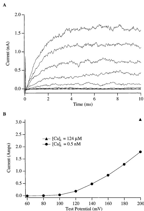
FIGURE 8. mslo currents at very low [Ca] i . (A) Currents were elicited with depolarizing steps to test potentials ranging from +60 to +200 mV in 20-mV increments. V hold = -50 mV. Included in the internal solution was 5 mM EGTA. No HEDTA or Ca 2+ was added. The calculated free [Ca] i in this solution was ~0.5 nM assuming contaminant Ca 2+ of 10 to 20 μM (see MATERIALS AND METHODS). The traces displayed are the average from 5 series recorded consecutively. (B) Peak current values from the data in A are plotted as a function of membrane voltage (●). Also included is the peak current measured from the same patch with a step to +200 mV while the patch was superfused with 124 μM [Ca] i (▲).
