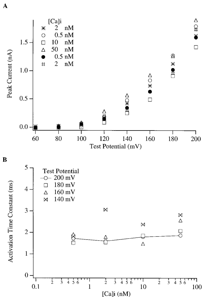
FIGURE 11. mslo currents are insensitive to changes in [Ca]_i in the low nanomolar range. (A) mslo currents recorded from a single membrane patch at the indicated [Ca]_i . Internal solutions were prepared from the standard solution as follows: 0.5 nM (no added Ca^{2+} , 5 mM EGTA), 2 nM (no added Ca^{2+} , 1 mM EGTA), 10 nM (0.28 mM added CaCl_2 , 5 mM EGTA), 50 nM (1.18 mM added CaCl_2 , 5 mM EGTA). The order of solution presentation was as follows 2 nM (*), 0.5 nM (○), 10 nM (□), 50 nM (△), 0.5 nM again (●), 2 nM again (#). (B) Time constants of activation for currents in A are plotted as a function [Ca]_i . Each symbol represents data from a different test potential as indicated. The data points at +200 mV have been connected (solid line). Time constants were determined by fitting the time course of activation with a single exponential function.
