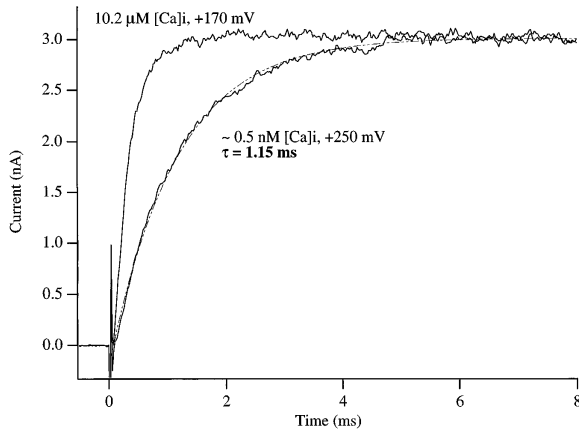
FIGURE 10. Rapid activation of mslo currents at very low [Ca]_i . The two current traces displayed were recorded from the same membrane patch with 10.2 \mu M and \sim 0.5 nM [Ca]_i (5 mM EGTA no added Ca^{2+} ) as indicated. The traces shown represent the average of 5 (10.2 \mu M [Ca]_i ) and 8 ( \sim 0.5 nM [Ca]_i ) traces recorded in consecutive current families. Voltage steps were from -100 to +170 mV at 10.2 \mu M [Ca]_i , and from 0 to +250 mV at \sim 0.5 nM [Ca]_i . The \sim 0.5 nM [Ca]_i trace was fitted with a single exponential function with a time constant of 1.15 ms. The fit is superimposed on the data (dashed line).
