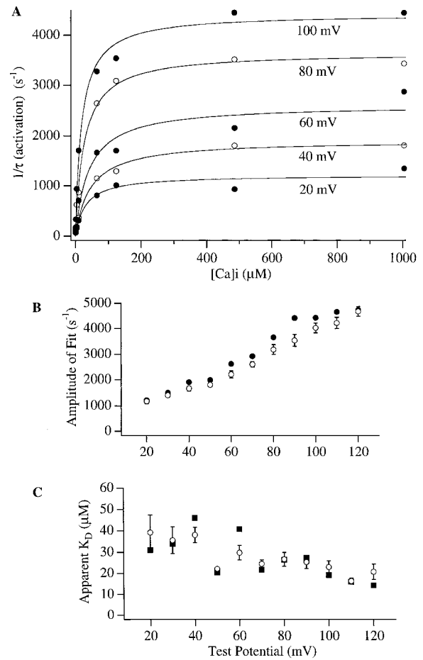
FIGURE 7. (A) The mslo macroscopic activation rate constant ( 1/\tau ) is plotted as a function of [Ca]_i for several different membrane voltages. Data are from a single membrane patch. Macroscopic rate constants were determined from exponential fits to the time course of activation. Voltages descend from top to bottom as indicated. Alternating open and closed markers have been used for ease of distinguishing data at differing voltages. Each data set has been fitted (solid curve) with the function 1/\tau = Amp/[1 + (K_D/[Ca]_i)] . To minimize the effects of outlying points an absolute, sum of squares criteria was used in fitting. The parameters from these fits, Amp (maximum macroscopic rate constant), and K_D (apparent Ca^{2+} dissociation constant) are plotted as a function of membrane voltage in B and C (●). Also included in B and C are mean values from 5 experiments (○). Error bars represent standard errors of the mean.
