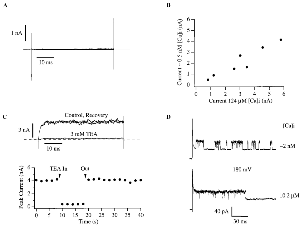
FIGURE 9. Currents recorded at high voltage and very low [Ca]_i are passing through mslo channels. (A) Control currents recorded from an oocyte not injected with RNA. Currents shown were elicited with 50-ms voltage steps to potentials ranging from +60 to +200 mV in 20-mV increments. V_{hold} = -50 mV. (B) Correlation between the amplitudes of mslo currents recorded from the same patches with \sim 0.5 nM ( ordinate ) or 124 \mu M ( abscissa ) [Ca]_i . Each symbol represents an individual experiment. Amplitudes were measured at the end of 50-ms depolarizations to +200 mV. V_{hold} = -50 mV (0.5 nM [Ca]_i ); V_{hold} = -120 mV (124 \mu M [Ca]_i ). (C) Current traces recorded from an outside out membrane patch with voltage steps to from -50 to +200 mV before ( control ), during (3 mM TEA), and after ( recovery ) exposure of the external surface of the patch to 3 mM TEA. In the
