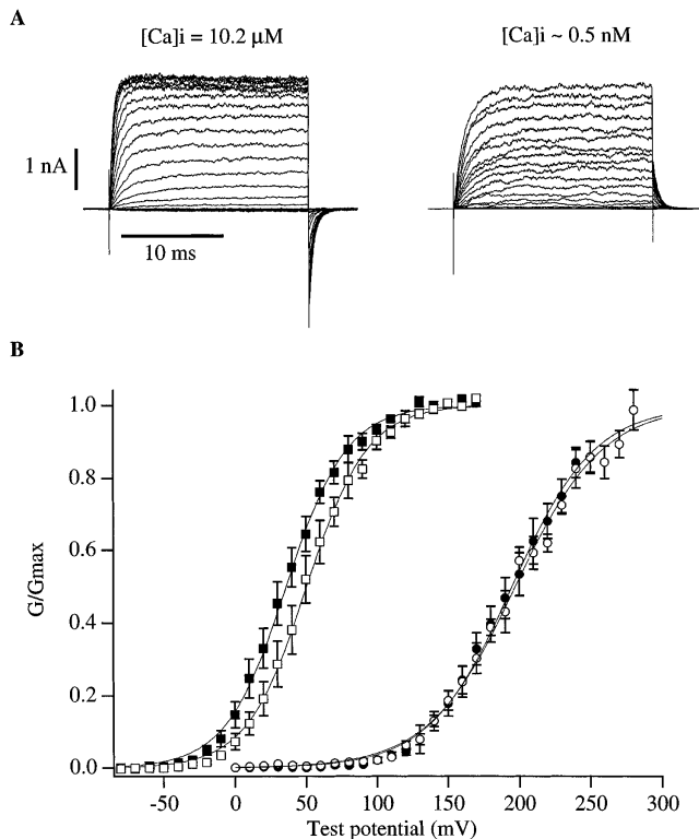
FIGURE 12. (A) mslo current families recorded from the same membrane patch at 10.2 \mu\text{M} and \sim 0.5 nM [\text{Ca}]_i . Each family displayed is the average of 5 (10.2 \mu\text{M} ) and 8 ( \sim 0.5 nM) families recorded in succession. (B) Mean mslo G-V curves recorded from 6 membrane patches with 10.2 \mu\text{M} [\text{Ca}]_i before (■) and after (□) superfusion with \sim 0.5 nM [\text{Ca}]_i (●). In three patches current families were determined with \sim 0.5 nM [\text{Ca}]_i with voltages up to +280 mV (○). Error bars represent standard errors of the mean. G-V curves were fit with the Boltzmann function G = G_{\text{max}}(1/[1 + e^{-(V-V_{1/2})zF/RT}]) and then normalized to the maximum of the fit. Fit parameters were as follows: (■) V_{1/2} = 36 mV, z = 1.18 ; (□) V_{1/2} = 50 mV, z = 1.19 ; (●) V_{1/2} = 195 mV, z = 0.87 ; (○) V_{1/2} = 197 mV, z = 0.83 .
