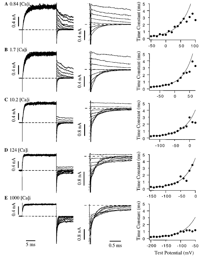
FIGURE 3. Deactivation of mslo currents. (A–E) Tail current families recorded from a single membrane patch. [Ca]_i were as indicated (top to bottom): 0.84, 1.7, 10.2, 124, and 1,000 \mu M . Each family displayed is the average of 4 series recorded consecutively under identical conditions. Depolarizations are for 20 ms. Repolarizations are for 10 ms. In the left panels complete series are displayed. The voltage increment is 10 mV. In the middle panels subsets of traces from the left have been expanded and fitted with single exponential functions (dashed curves). The voltage increment is 20 mV. In the right panels are displayed plots of the deactivation time constant as a function of test potential. The most hyperpolarized portions of these curves are fitted with the function \tau = Ae^{qV/RT} + b (solid curves). (A) 0.84 \mu M [Ca^{2+}]_i : prepulse potential: 180 mV. Test potentials: -50 to 100 mV, q = 0.62 , b = 0.069 . (B) 1.7 \mu M [Ca^{2+}]_i : prepulse potential: 160 mV. Test potentials: -80 to 70 mV, q = 0.74 , b = 0.223 . (C) 10.2 \mu M [Ca^{2+}]_i : prepulse potential: 100 mV. Test potentials: -130 to 30 mV, q = 0.67 , b = 0.176 . (D) 124 \mu M [Ca^{2+}]_i : prepulse potential: 80 mV. Test potentials: -150 to 20 mV, q = 0.68 , b = 0.226 . (E) 1,000 \mu M [Ca^{2+}]_i : prepulse potential: 50 mV. Test potentials: -200 to -50 mV, q = 0.67 , b = 0.163 .
