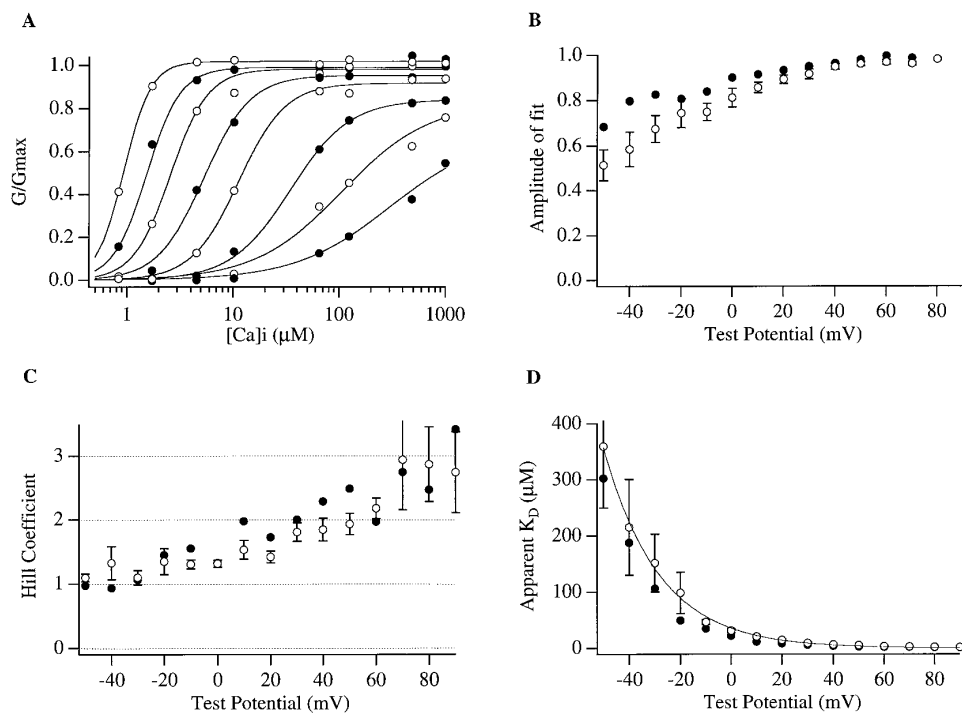
FIGURE 13. Ca-dependence of mslo currents. (A) Conductance vs. voltage (G-V) relations at the following [\text{Ca}]_i : 0.84, 1.7, 4.5, 10.2, 65, 124, 490, 1,000 \mu\text{M} where constructed from tail current amplitudes measured 0.2-ms after repolarization from the appropriate test potential to -80 mV. Each G-V curve was then fitted with a Boltzmann function and normalized to the maximum of the fit. These data were transformed to dose-response form for each voltage and displayed in A. Smooth curves represent fits to the Hill equation G/G_{\text{max}} = \text{Amp}/\{1 + (K_D/[\text{Ca}])^n\} , where n = Hill coefficient, and K_D = apparent \text{Ca}^{2+} dissociation constant. Voltages descend from left to right starting at +90 mV and ending at -50 mV in 20-mV increments. Alternating open and closed markers have been used for ease of distinguishing data at differing voltages. The data are from the same membrane patch.
