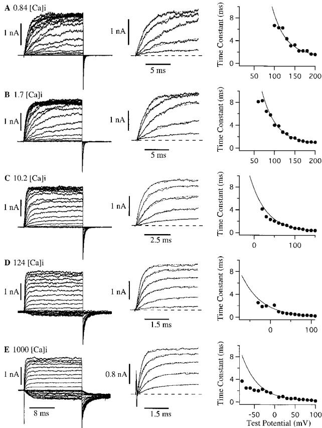
FIGURE 2. Activation of mslo currents. (A–E) Current traces from a single membrane patch recorded after a series of depolarizations to increasingly more positive membrane voltages. [Ca]_i were as indicated (top to bottom) 0.84, 1.7, 10.2, 124, and 1,000 \mu M . Each series displayed is the average of 4 series recorded consecutively under identical conditions. Depolarizations were for 20 ms. Repolarizations were to -80 mV. In the left panels complete series are displayed. The voltage increment is 10 mV. In the middle panels a subset of traces have been expanded and fitted with single exponential functions (dashed curves). The voltage increment is 20 mV. In the right panels are shown plots of activation time constants as a function of test potential. The later portions of these curves are fitted with the function \tau = Ae^{qV/RT} + b (solid curves). (A) 0.84 \mu M [Ca]_i , V_{hold} = -50 mV: (left) depolarizations ranged from 0 to +200 mV. (middle) Depolarizations ranged from +80 to +160 mV; (right) fit parameters: range +130 to 200 mV, q = 0.77 , b = 1.3 ms. (B) 1.7 \mu M [Ca]_i , V_{hold} = -80 mV: (left) depolarizations ranged from -40 to +200 mV in 10-mV increments; (middle) depolarizations ranged from +60 to +140 mV; (right) fit parameters: range +90 to +150 mV, q = 0.63 , b = 0.16 ms (D) 124 \mu M [Ca]_i , V_{hold} = -120 mV: (left) depolarizations ranged from -120 to +110 mV; (middle) depolarizations ranged from +10 to +110 mV; (right) fit parameters: range -10 to +110 mV, q = 0.52 , b = 0.01 ms. (E) 1,000 \mu M [Ca]_i , V_{hold} = -180 mV: (left) depolarizations ranged from -180 to +100 mV; (middle) depolarizations ranged from +20 to +100 mV; (right) fit parameters: range -10 to +100 mV q = 0.64 , b = 0.23 ms.
