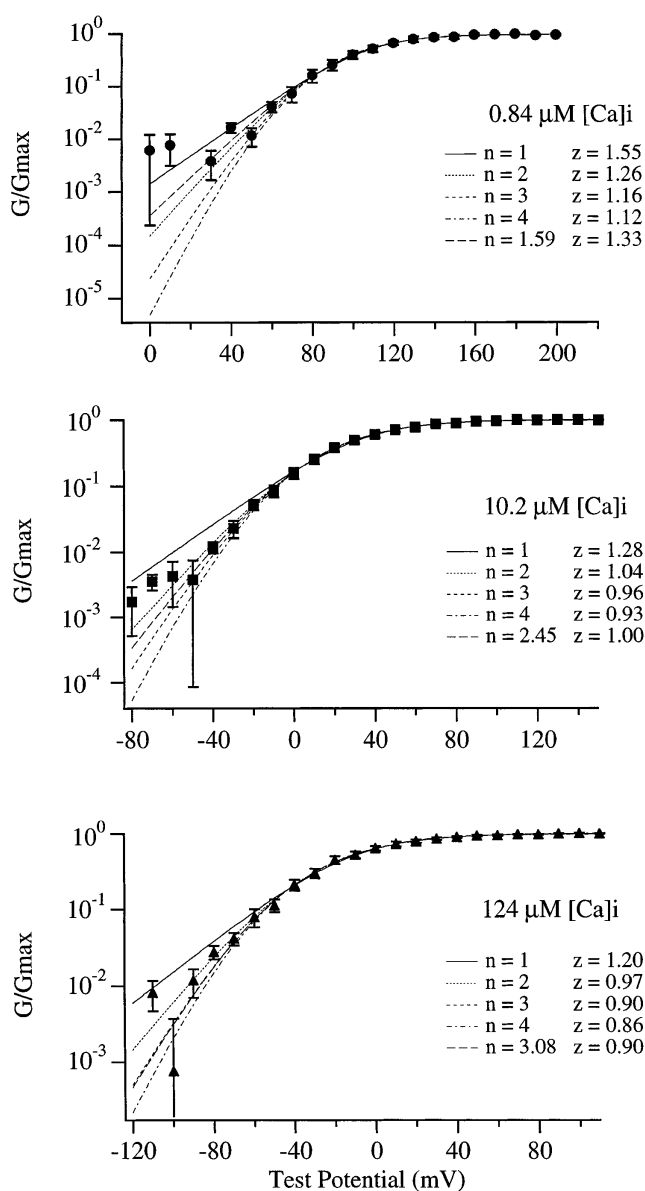
FIGURE 14. mslo G-V relations fitted with Boltzmann functions raised to powers between 1 and 4. Displayed are semi-log plots of the mslo G-V relation determined with 0.84 (A), 10.2 (B), and 124 (C) \mu M [Ca]_i . Each data set represents the mean of from 5 to 8 experiments. These data are the same as that displayed in Fig. 5 B. Each curve has been fitted with the function G/G_{max} = A[1/(1 + e^{-(V-V_{1/2})zF/RT})]^n . Curves corresponding to the best fit with n = 1, 2, 3, and 4 have been superimposed on the data. For each [Ca]_i a fit with n varying freely is also displayed. The line type indicating n , as well as the fit parameter z , are as indicated on the figure.
