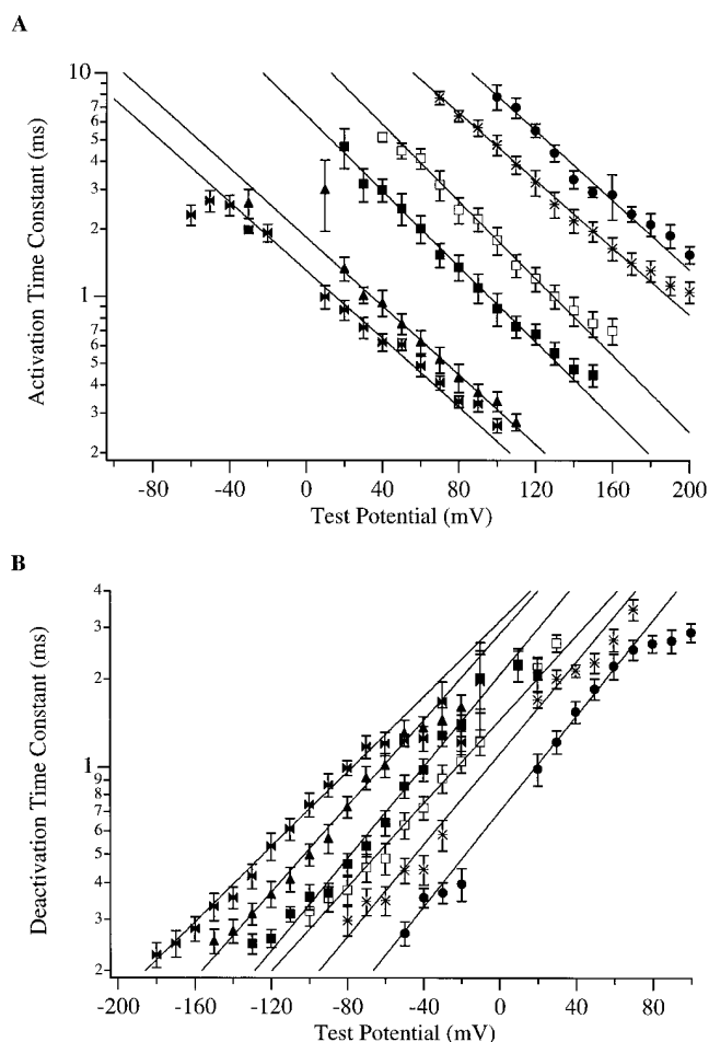
FIGURE 4. Mean activation and deactivation time constant as a function of both voltage and [\text{Ca}]_i . Displayed are semi-log plots of activation (A) and deactivation (B) time constants. Each curve represents the mean of between 4 and 10 experiments. Error bars indicate standard errors of the mean. Solid lines represent fits to the function \tau = Ae^{-qFV/RT} . Fits were done by eye. Fit parameters: (A) [\text{Ca}]_i = 0.84 \mu\text{M} ( \bullet ), n = 4 , q = 0.46 ; [\text{Ca}]_i = 1.7 \mu\text{M} (*), n = 10 , q = 0.44 ; [\text{Ca}]_i = 4.5 \mu\text{M} ( \square ), n = 9 , q = 0.51 ; [\text{Ca}]_i = 10.2 \mu\text{M} ( \blacksquare ), n = 7 , q = 0.50 ; [\text{Ca}]_i = 124 \mu\text{M} ( \blacktriangle ), n = 7 , q = 0.45 ; [\text{Ca}]_i = 1,000 \mu\text{M} ( \blacktriangleright ), n = 5 , q = 0.45 . (B) [\text{Ca}]_i = 0.84 \mu\text{M} ( \bullet ), n = 7 , q = -0.48 ; [\text{Ca}]_i = 1.7 \mu\text{M} (*), n = 6 , q = -0.46 ; [\text{Ca}]_i = 4.5 \mu\text{M} ( \square ), n = 7 , q = -0.42 ; [\text{Ca}]_i = 10.2 \mu\text{M} ( \blacksquare ), n = 10 , q = -0.46 ; [\text{Ca}]_i = 124 \mu\text{M} ( \blacktriangle ), n = 9 , q = -0.43 ; [\text{Ca}]_i = 1,000 \mu\text{M} ( \blacktriangleright ), n = 10 , q = -0.38 .
