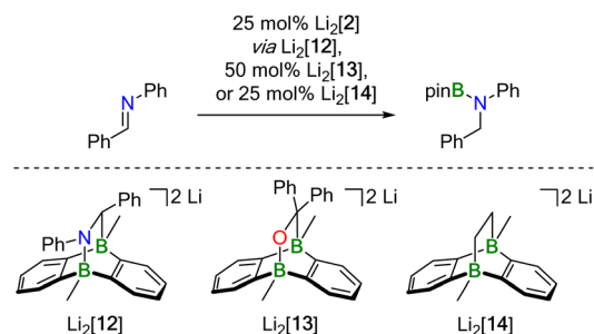
Scheme 4 Crossover experiment to demonstrate that hydroboration of Ph(H)C=NPh with HBpin can be mediated not only by Li 2 [2] (actual catalyst: Li 2 [12]), but also by pre-formed Li 2 [13] or Li 2 [14] without generating Ph 2 (H)C–OBpin or H 3 C–CH 2 Bpin as crossover side product, respectively (THF- d 8 , room temperature). Note that the high catalyst loadings were used for the sole purpose of being able to detect any catalyst degradation or trace formation of crossover products by NMR spectroscopy.
