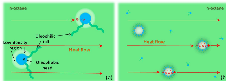
Figure 3. Schematics of the thermal transport in AOT solutions with AOT loading below (a) or above (b) CMC. (a) The interfacial region between AOT's hydrophilic headgroup and the apolar octane molecules hinders the thermal transport near the headgroup, and thus reduces the thermal conductivity of the solution. (b) The hydrogen bonding network among the adsorbed water molecules and the AOT's hydrophilic headgroups can provide a rapid thermal transport pathway and thus help increase the thermal conductivity of the micellar solution.
