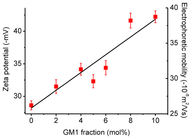
FIGURE 1 Influence of GM1 content on the electrophoretic mobility and \zeta potential of 2 mM POPC LUVs in 1 mM HEPES at 40°C. The error bars indicate standard error. To see this figure in color, go online.
