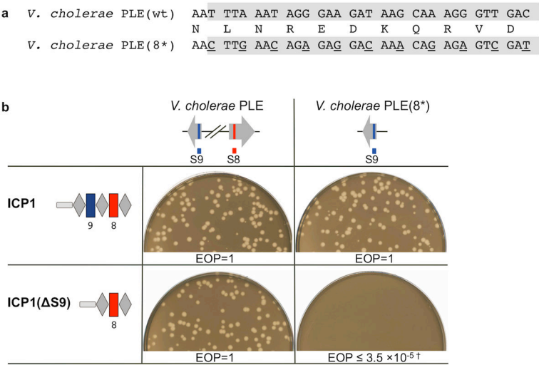
Figure 3. Sequence-based targeting by the ICP1 CRISPR/Cas system is essential for lytic growth on V. cholerae PLE + a , Disruption of the V. cholerae PLE target protospacer generating V. cholerae PLE(8*). The 32 bp protospacer sequence is shaded in grey. b , The sensitivity of each strain (top row) to ICP1 or ICP1 S9 (left column) is shown. Identity between the spacer and targeted protospacer is indicated by the red and blue rectangles. The efficiency of plaquing (EOP, which is the plaque count on the mutant host strain divided by that on the wild-type host strain) is indicated. A dagger indicates that the EOP is 10 -5 or 10 -8 depending on the presence of PLE in the host strain used for propagation as discussed in the text.
