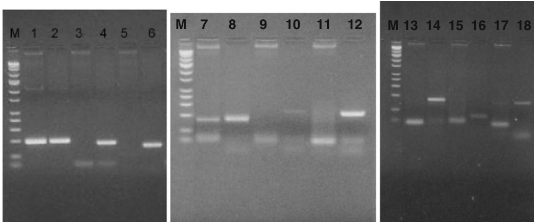
Fig. 2. PCR screening test for peanut immature pod-specific genes. PCR templates: peanut leaf cDNA library ( lanes 1, 3, 5, 7, 9, 11, 13, 15, 17 ) and peanut immature pod cDNA library ( lanes 2, 4, 6, 8, 10, 12, 14, 16, 18 ). PCR products: control gene (~194 bp; lanes 1 and 2 ); candidate genes that are only expressed in peanut pod: cluster 7 (~173 bp; lanes 3 and 4 ), cluster 31 (~152 bp; lanes 5 and 6 ), cluster 33 (~233 bp; lanes 9 and 10 ), cluster 15 (~218 bp; lanes 11 and 12 ), cluster 11 (~170 bp; lanes 13 and 14 ), cluster 8 (~80 bp; lanes 15 and 16 ); candidate genes that are more highly expressed in peanut immature pod than leaf: cluster 23 (~152 bp; lanes 7 and 8 ), cluster 24 (~160 bp; lanes 17 and 18 ). M DNA marker.
