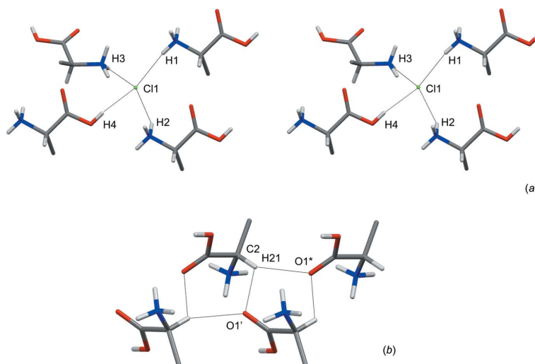
Figure 3 (a) Stereodrawing showing the coordination of hydrogen-bond donors around a Cl^- anion (see Table 2 for symmetry operators). (b) Tape motif along the b axis generated from C^\alpha-H\cdots O hydrogen bonds. O1* is at (x, y+1, z) , O1' at (-x+\frac{3}{2}, y+\frac{1}{2}, -z+1) . Side chains have been truncated beyond C^\beta .
