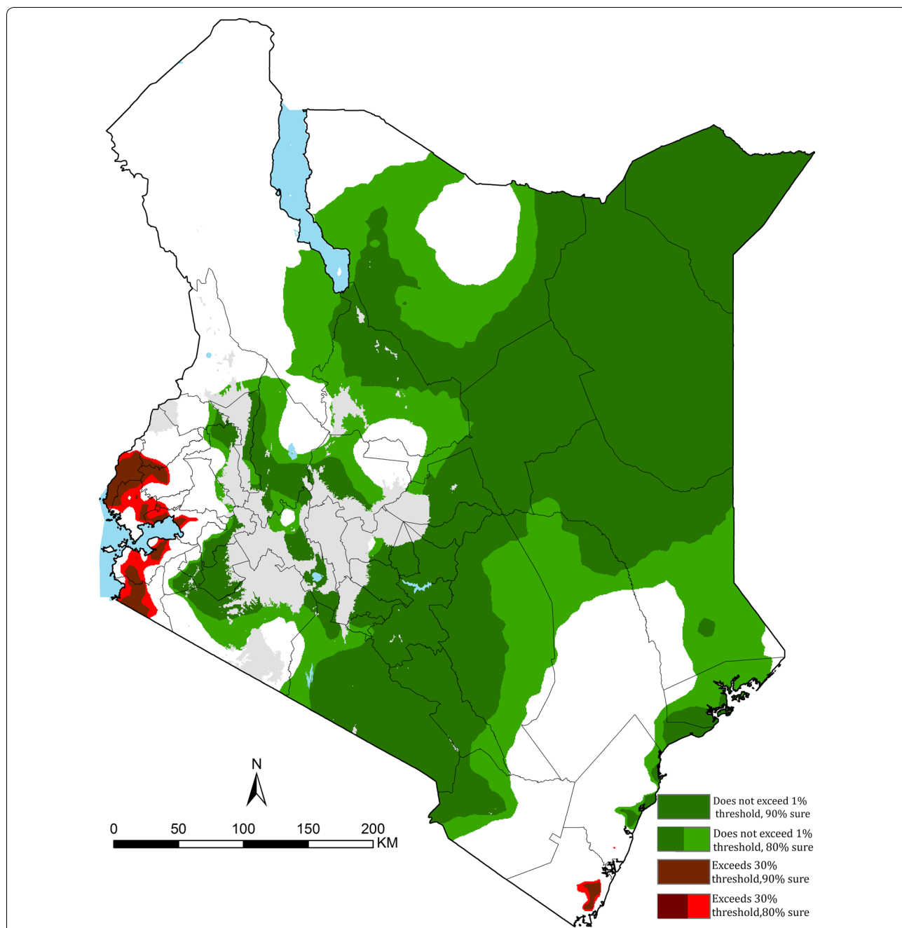
Fig. 5 Composite of 3 years 2013, 2014 and 2015 showing areas where predicted PPR_{2-10} is less (non-exceedance probability) than 1% which were > 80% confidently predicted (light green and dark green) or > 90% confidently predicted (dark green); and areas where PPR_{2-10} is greater (exceedance probability) than 30% which were > 80% confidently predicted (light red and dark red) or > 90% confidently predicted (dark red). Areas which do not support malaria transmission are shown in grey (see Fig. 1); all other areas where transmission can occur is shown in white
