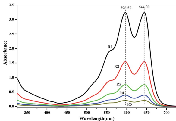
Fig. 2 Absorption spectra of different NH-blue-OH concentrations in THF solution.
