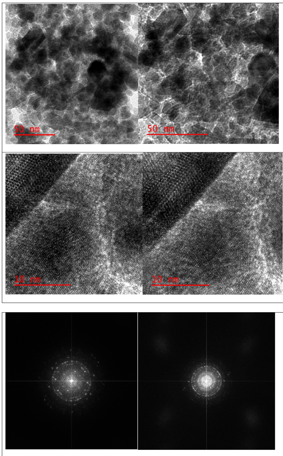
Fig. 3 TEM image of \text{Fe}_3\text{O}_4@\text{CPTMS}@\text{guanidine}-\text{BuSO}_3\text{H} MNPs.
