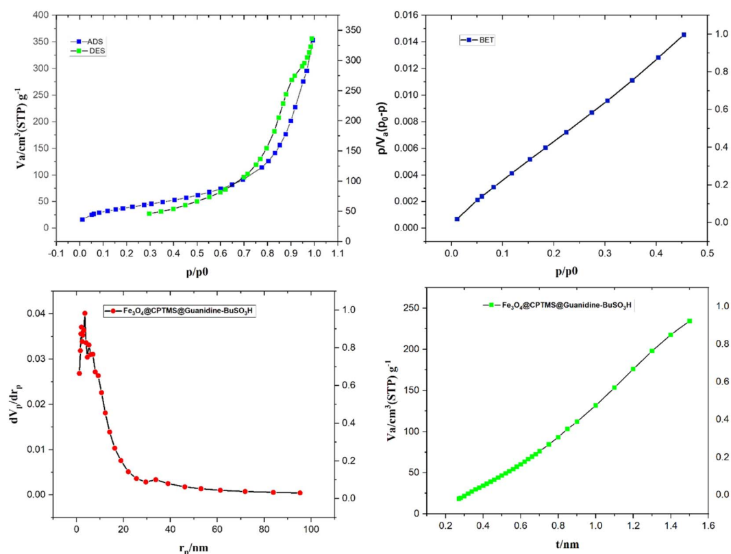
Fig. 6 The nitrogen adsorption–desorption isotherm and pore size distribution of \text{Fe}_3\text{O}_4@\text{CPTMS}@ guanidine- \text{BuSO}_3\text{H} MNPs.
