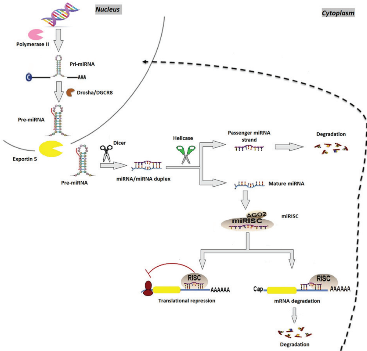
Figure 1. miRNA biosynthesis. miRNA genes are transcribed by RNA polymerase II as pri-miRNAs, which are subsequently processed by Drossha, resulting in pre-miRNA. Pre-miRNAs are then transported by the exportin 5-Ran GTPase shuttle system into the cytoplasm where they are cleaved by another RNase family enzyme (Dicer), resulting in the miRNA/miRNA duplex. During this phase, Dicer interacts with AGO2 proteins generating the RISC. Immediately following this, one strand of the miRNA duplex is removed while the single stranded miRNA remains in the complex and interacts with the 3' untranslated region of target mRNA genes, inducing posttranscriptional silencing and translational repression. miRNA, microRNA; pri-miRNA, primary RNA; pre-miRNA, miRNA precursor; DGCR8, DiGeorge syndrome critical region 8; AGO2, argonaute 2; RISC, RNA-induced silencing complex.
