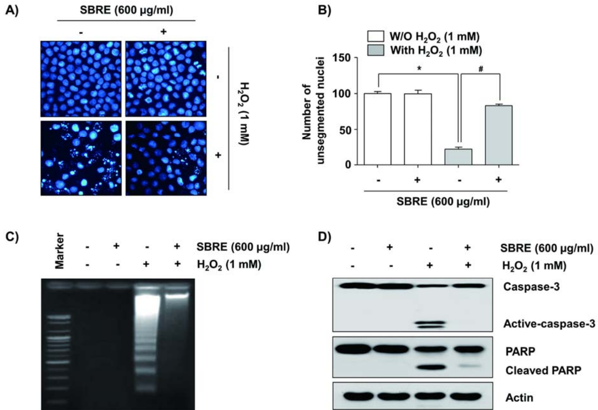
Figure 6: Prevention of H 2 O 2 -induced chromatin condensation, DNA fragmentation, cleavage of caspase-3 and degradation of PARP by SBRE in HaCaT keratinocyte cells. Cells were pretreated with 600 µg/ml for 1 h and then stimulated with or without 1 mM µM H 2 O 2 for 24 h. (A and B) The cells were fixed and stained with DAPI solution. After 15 min incubation at room temperature, stained nuclei were observed using a fluorescence microscope (original magnification, 400x). Each point represents the mean ± SD of three independent experiments (*P < 0.05 vs. untreated control; #P < 0.05 vs. H 2 O 2 -treated cells). (C) DNA fragmentation was analyzed by extracting the fragmented DNAs and separating them by electrophoresis in a 1.0 % agarose gel containing EtBr. (D) The cells were lysed and then equal amounts of cell lysates were separated on SDS-polyacrylamide gels and transferred to nitrocellulose membranes. The membranes were probed with specific antibodies against caspase-3 and PARP, and the proteins were visualized using an ECL detection system. Actin was used as an internal control.
