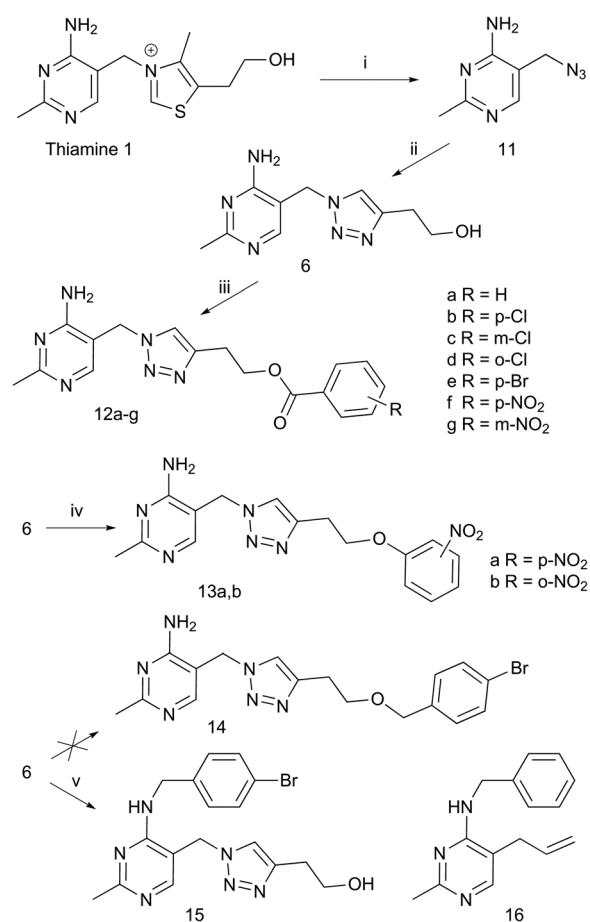
Scheme 1 Synthesis of analogues 12, 13 and 15. Reagents and conditions: (i) NaN_3 , Na_2SO_3 , H_2O , 65 °C; (ii) 3-butyn-1-ol, CuSO_4 \cdot 5H_2O , sodium ascorbate, t -BuOH, H_2O , RT; (iii) ArCO_2H , DCC, DMAP, DMF, RT; (iv) 2- or 4-fluoronitrobenzene, KHMDS, NMP, RT; (v) 4-bromobenzyl bromide, KHMDS, NMP, 45 °C. 16 is a similar compound to 15 on ChEMBL with reported antiplasmodial activity.
