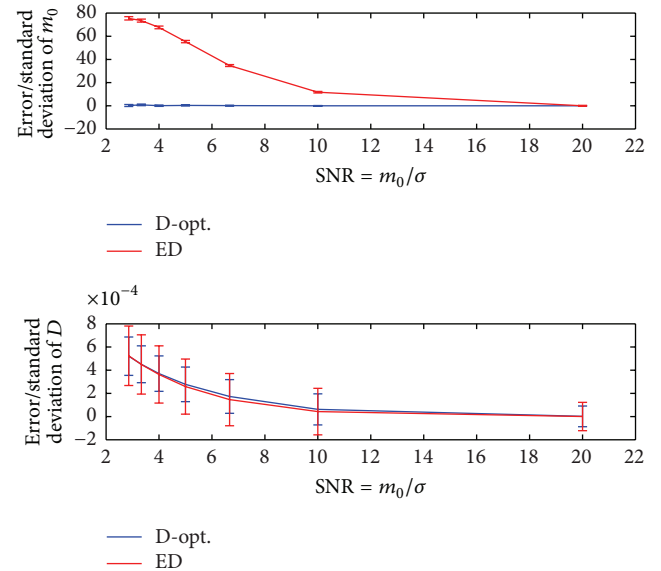
FIGURE 8: Error and standard deviation of \widehat{D} and \widehat{m}_0 as a function of SNR (defined as m_0/\sigma_G ), where D = 1 \times 10^{-3} , N = 10 , b_{\min} = 0 , b_{\max} = 2000 , m_0 = 500 , and N_{MC} = 20000 . The D-optimal design is compared to the ED design.
