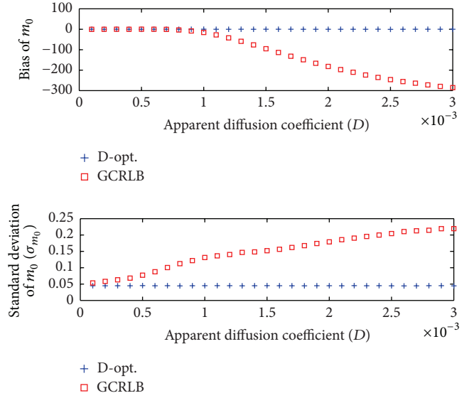
FIGURE 4: Bias and standard deviation of the estimated m_0 values for a range of D values, where N = 10 , b_{\min} = 0 , b_{\max} = 1500 , m_0 = 500 , N_{MC} = 20000 , and \text{SNR} = m_0/\sigma_G = 10 . The proposed D-optimal method is compared to GCRLB [23].
