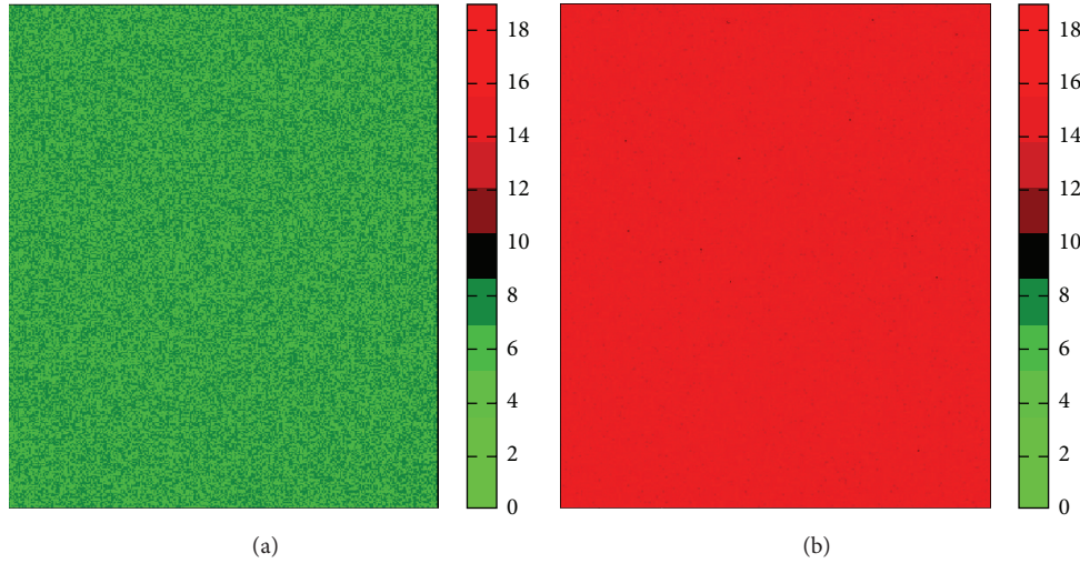
FIGURE 11: Standard deviation in estimation of \widehat{m}_0 . The D-optimal design (a) produces more precise estimates compared to the ED design (b). Note that the standard deviation is multiplied by 100 to enhance the visualization.
