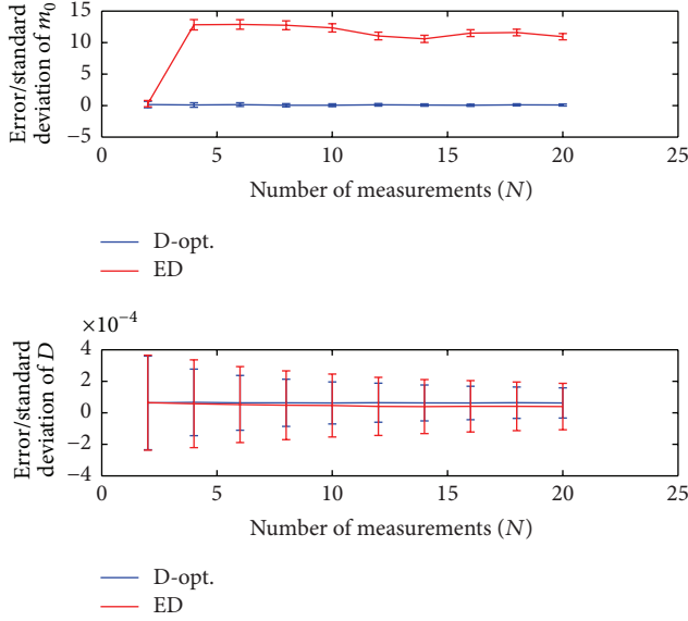
FIGURE 6: Error and standard deviation of \widehat{D} and \widehat{m}_0 for the range N = 2 to N = 20 , where D = 1 \times 10^{-3} , b_{\min} = 0 , b_{\max} = 2000 , m_0 = 500 , N_{MC} = 20000 , and \text{SNR} = m_0/\sigma_G = 10 . The D-optimal design is compared to the ED design.
