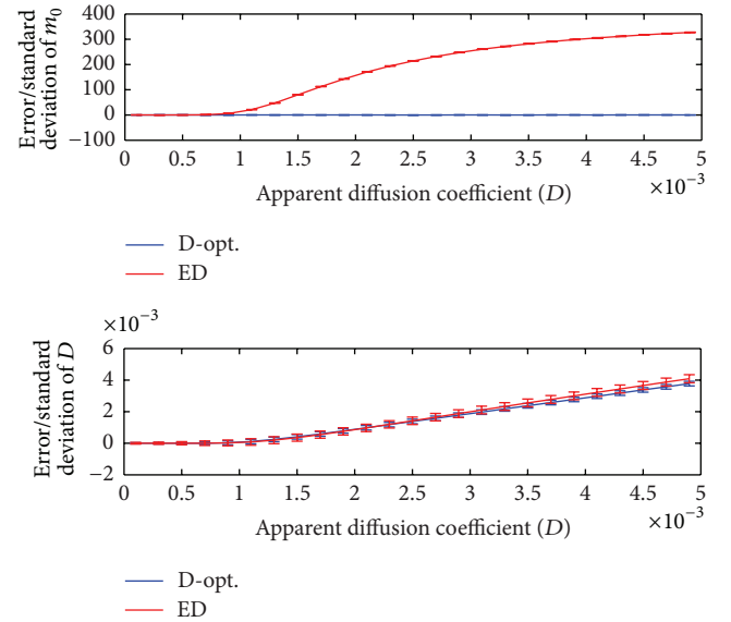
FIGURE 5: Error and standard deviation of \widehat{D} and \widehat{m}_0 for the range D \in [0.1, 5] \times 10^{-3} , where N = 10 , b_{\min} = 0 , b_{\max} = 2000 , m_0 = 500 , N_{MC} = 20000 , and \text{SNR} = m_0/\sigma_G = 10 . The D-optimal design is compared to the ED design (where b_i s are equidistantly distributed between b_{\min} and b_{\max} ).
