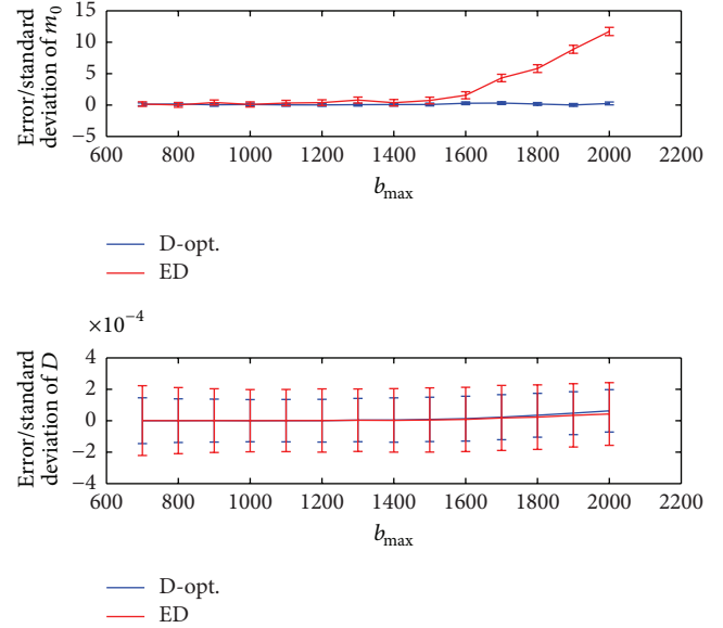
FIGURE 7: Error and standard deviation of \widehat{D} and \widehat{m}_0 as a function of b_{\max} , where D = 1 \times 10^{-3} , N = 10 , b_{\min} = 0 , m_0 = 500 , N_{MC} = 20000 , and \text{SNR} = m_0/\sigma_G = 10 . The D-optimal design is compared to the ED design.
