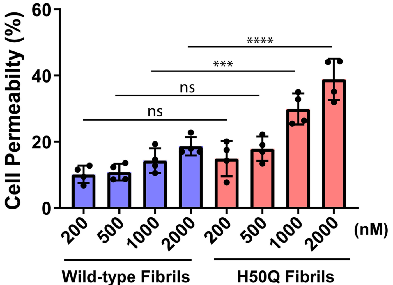
Extended Data Fig. 8. H50Q fibrils disrupt PC12 cell membranes more than WT fibrils Differentiated PC12 cells were treated with sonicated WT and H50Q fibrils and cell permeability was measured via LDH activity in the media (see Methods). H50Q leads to significantly higher cell permeabilization at 1000 and 2000 nM than WT a-syn. Error bars represent standard deviation of four independent experiments. **** = p-value 0.0001. *** = p-value 0.001. ns = p-value > 0.05. P-values were calculated using an unpaired, two-tailed t-test with a 95% CI.
