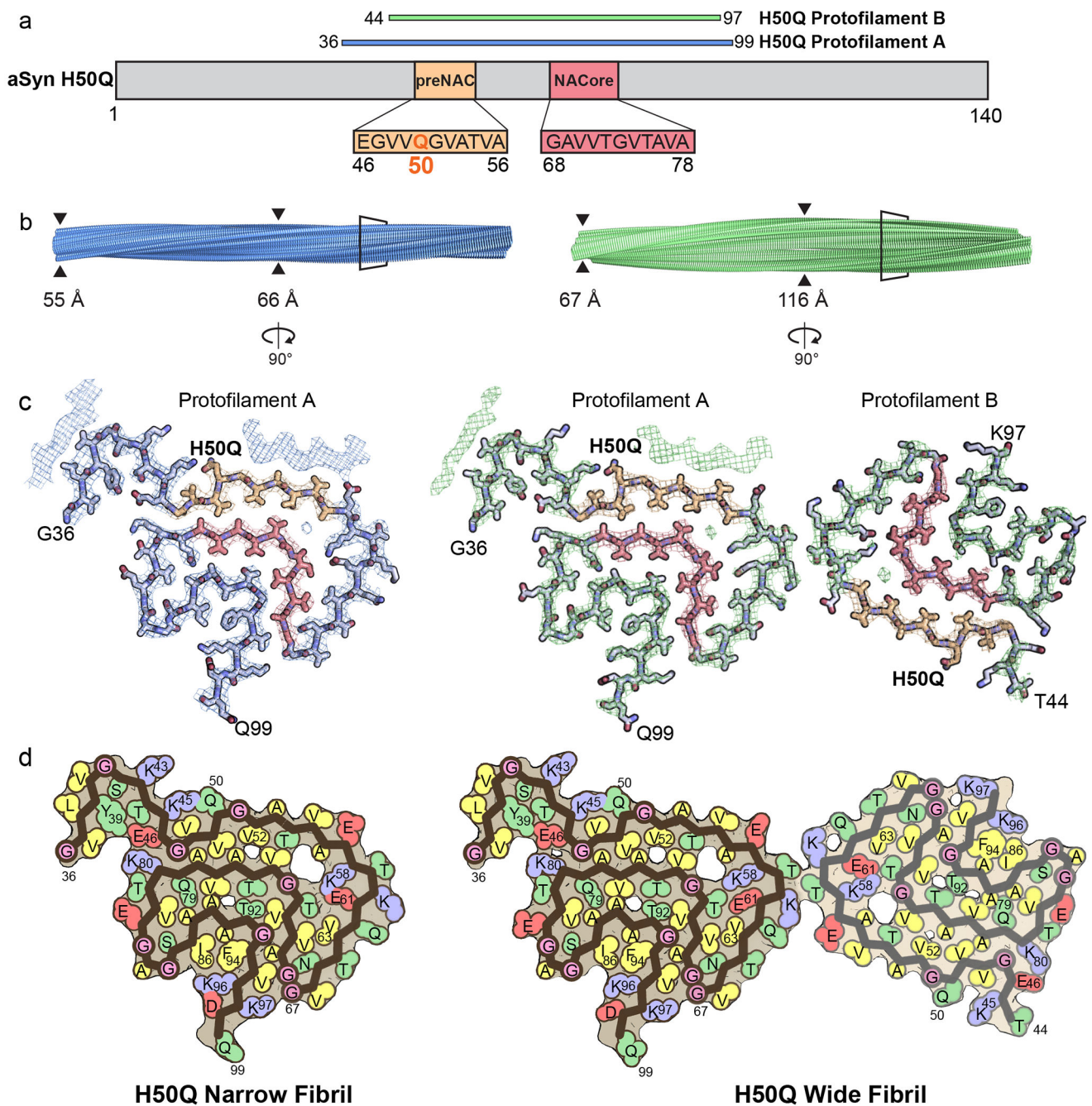
Figure 2. Cryo-EM Structures of H50Q Polymorphs
