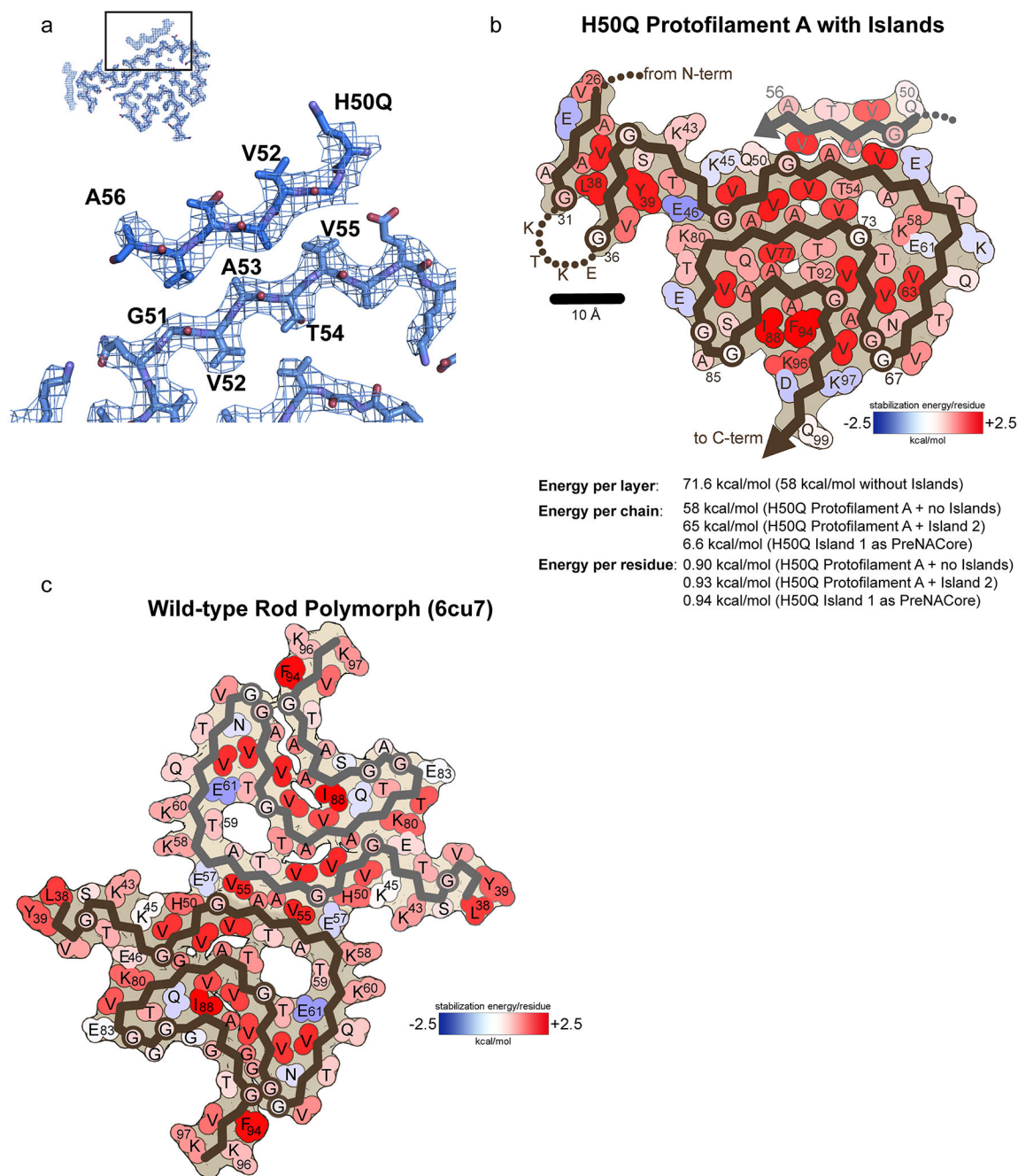
Extended Data Fig. 5. PreNAC homozipper Island 1 model and additional solvation energy maps a) Speculative model of preNAC residues 50 QGVATVA 56 occupying Island 1 in Protofilament A. b) Atomic solvation map and energetic calculations for Protofilament A with Island 1 as 50 QGVATVA 56 and Island 2 as 26 VAEAAG 31 . c) Atomic energy solvation map for Wild-type rod polymorph (6cu7). Notice that K58 and T59 can have favorable stabilization energies whether they are facing the solvent or facing the cavity in the \beta -arch.
