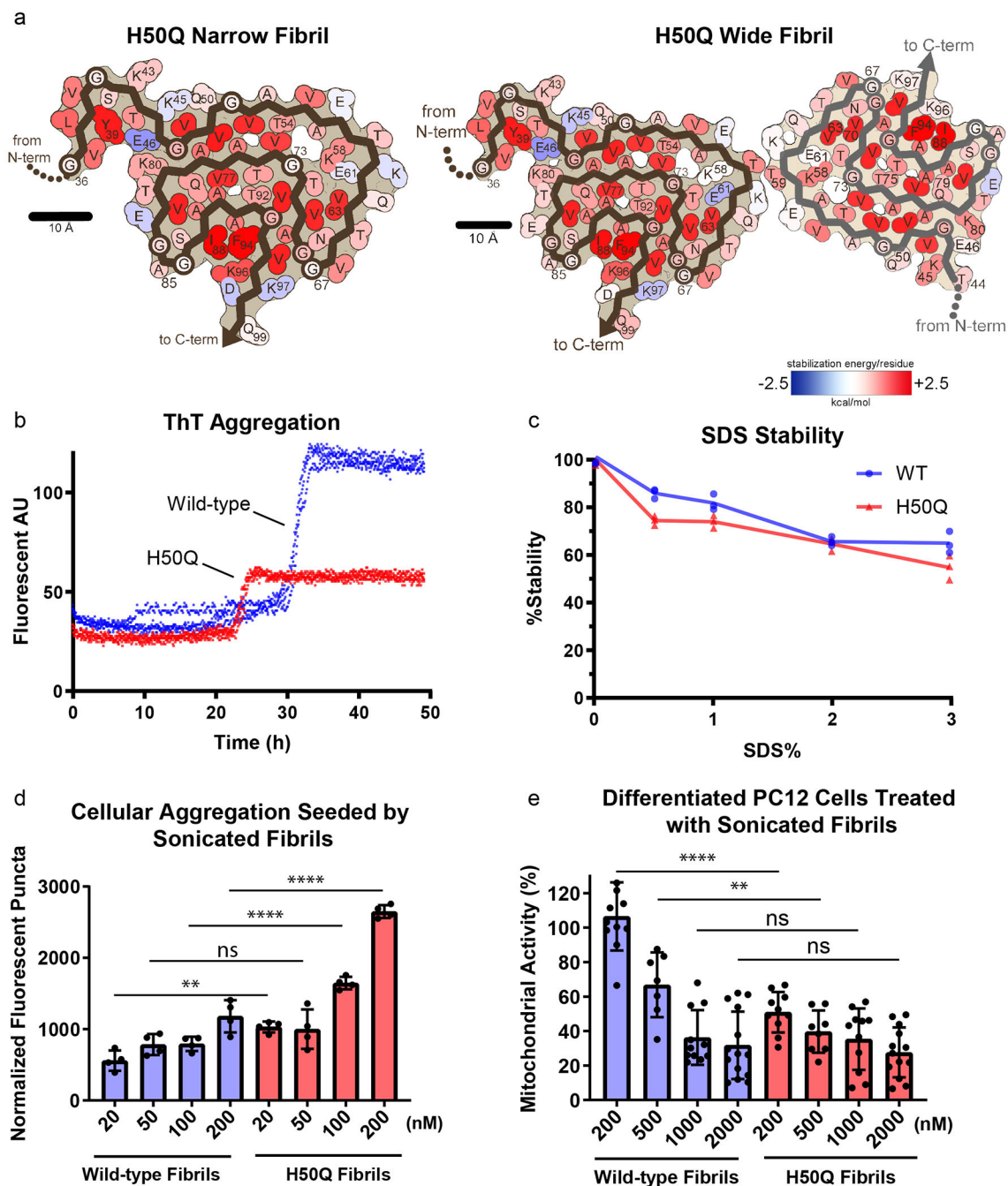
Figure 4. Solvation energy maps and biochemical characterization of H50Q and wild-type \alpha -syn. a) Solvation energy maps of H50Q Narrow and Wide Fibrils. The stabilizing residues are red; the de-stabilizing residues are blue. b) ThT assay measuring kinetics of H50Q and wild-type \alpha -syn aggregation. Data from three independent replicates for each sample are shown for each time point. Wild-type aggregation plateaus at 30 h whereas H50Q aggregates faster and plateaus at 23 h. c) Stability assay of H50Q and wild-type \alpha -syn. Fibrils were brought to the indicated concentration of SDS and heated at 70° C for 15 minutes before ThT signal
