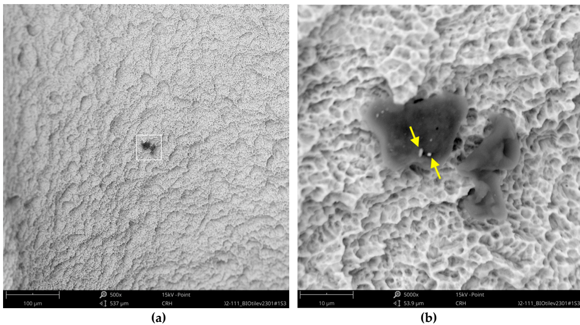
Figure 15. Bioconcept implant with organic particles (10–15 \mu\text{m} ); (a) red marked area in Figure 13, SEM 500 \times ; (b) magnification (5000 \times ) of white marked area in the left image (a); arrows indicate two embedded metal particles (0.5–1 \mu\text{m} ) showing significant iron signals in the subsequent EDS differential measurement.
