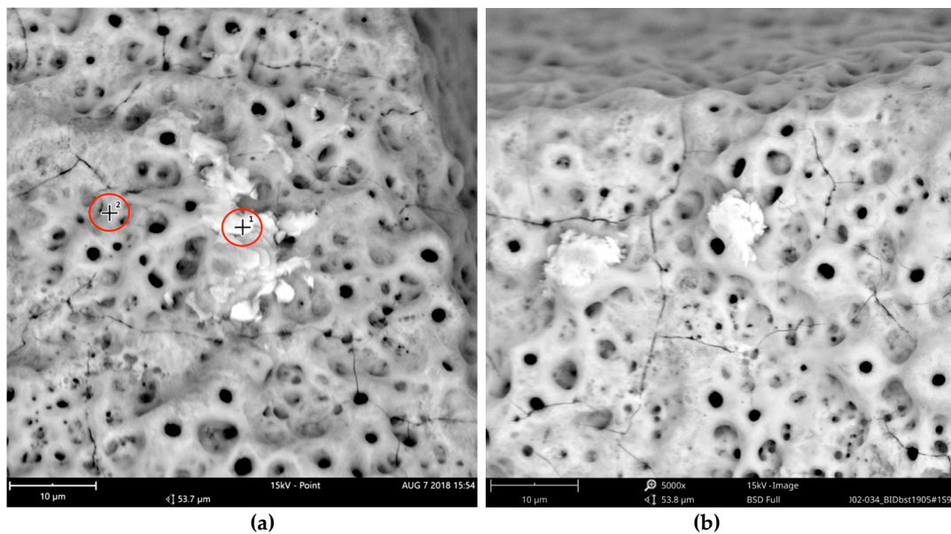
Figure 21. Aluminum-containing particles (5–10 μm) on the surface of the Biodenta implant; location shown using yellow arrows in Figure 19; (a) SEM 5000× with 2 points of EDS spot measurement shown in Figure 22; (b) impurities with similar size in close proximity to particles shown in the left image (a).
