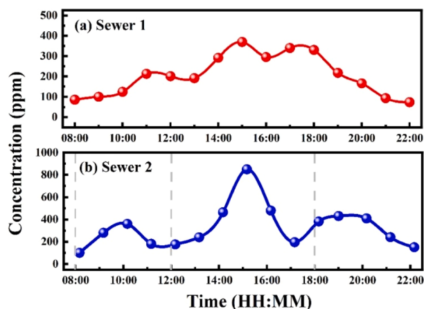
Fig. 8. Real-time \text{CH}_4 concentration monitoring at two sewer locations. (a) \text{CH}_4 concentration in Location 1 sewer. (b) \text{CH}_4 concentration in Location 2 sewer.
