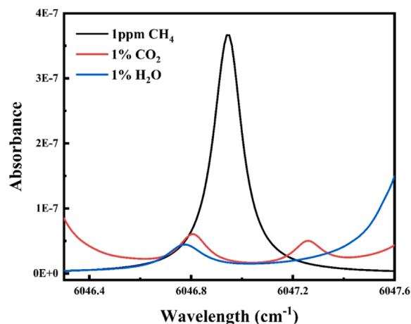
Fig. 9. \text{CH}_4 , \text{H}_2\text{O} and \text{CO}_2 absorbance spectra in the infrared region provided by the HITRAN database in the spectral range of 6046.3\text{ cm}^{-1} and 6047.6\text{ cm}^{-1} .
