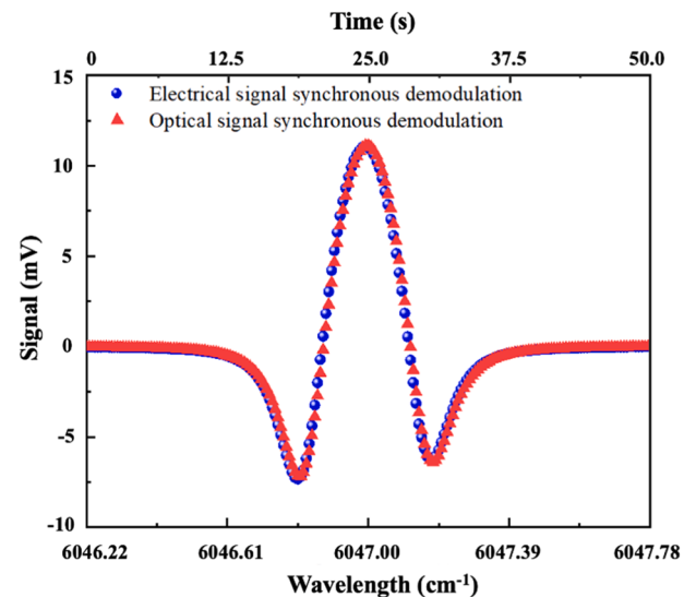
Fig. 5. Comparison of 1 % CH 4 /N 2 concentration measurements using conventional electrical signal demodulation technology and the proposed OSSD method.
