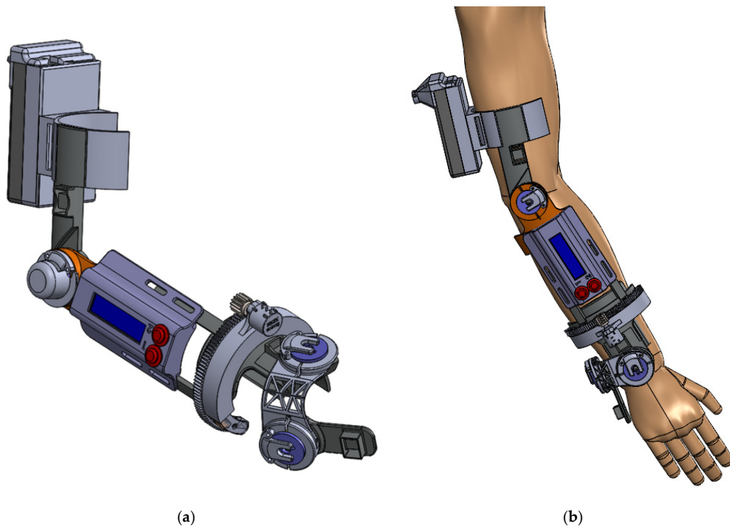
Figure 4. (a) 3D Modelling of the final prototype assembly, (b) Prototype mounted on the arm of a subject.
