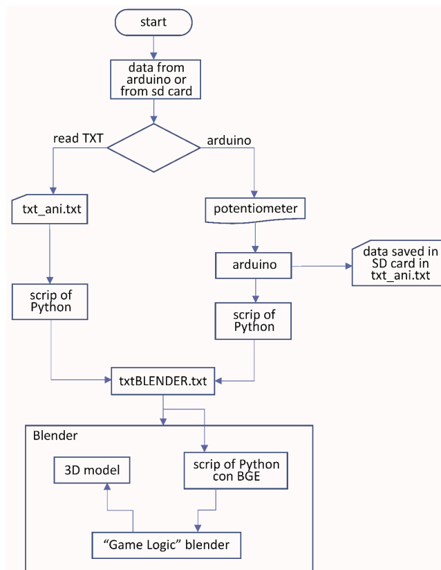
Figure 8. 3D animation data flowchart.
