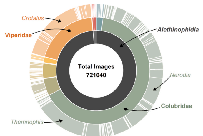
Fig. 1. Taxonomic structure of dataset. The innermost ring represents infra-orders: blindsnakes (Scolecophidia; light gray) and all other snakes (Alethinophidia; dark gray). The middle ring represents families, and the outermost ring represents genera. Width of slices is scaled to the number of photos.
