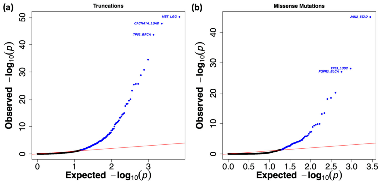
Fig. 3. QQ-plots of -\log_{10} adjusted genotype p -values from somatic truncations (a) and missense mutations (b) on likely driver genes in 32 cancer types. The red diagonal line is the expected value. Gene-cancer pairs showing significant associations ( P < 0.05 ) are marked in blue and the top three ranked pairs are labeled.
