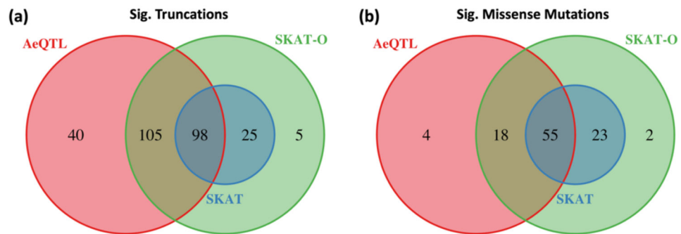
Fig. S3. Venn diagrams of significant associations identified by AeQTL, SKAT, and SKAT-O for (a) truncations and (b) missense mutations in TCGA somatic likely-driver-subset analysis.
