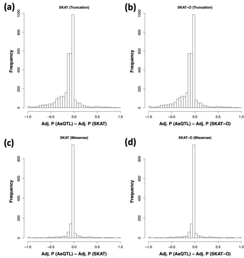
Fig. S2. Histograms of the differences between adjusted p -values from AeQTL and (a) SKAT for truncations, (b) SKAT-O for truncations, (c) SKAT for missense mutations, (d) SKAT-O for missense mutations in TCGA somatic likely-driver-subset analysis.
