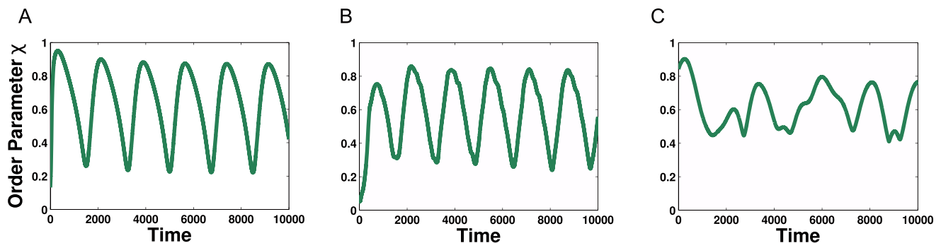
Figure 6. Kuramoto simulations for networks of clustered random networks Time series for global order parameter, with k = 0.4 (A), 0.1 (B), and 0.06 (C) showing multi-modal dynamics. The simulations are for networks described in Figure 5 and the parameter values taken from the oscillating regions. doi:10.1371/journal.pone.0075569.g006
