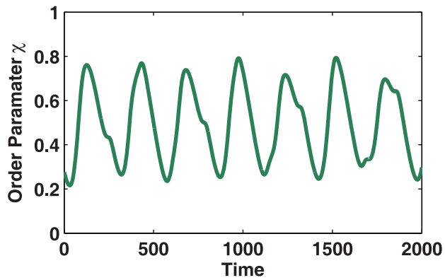
Figure 2. Kuramoto simulation for the network in Figure 1. Time series for order parameter, \chi , showing oscillatory dynamics for a network of Kuramoto oscillators coupled as in Figure 1. The coupling strength k=0.2 and the frequencies are normally distributed with standard deviation \sigma(\omega)=0.02 . Note, for such parameter values it is possible to observe full synchronisation or oscillating dynamics as shown above depending on the individual frequencies of the oscillators. The example demonstrated here, although fairly typical, is not the only observable dynamics for such a network. doi:10.1371/journal.pone.0075569.g002
