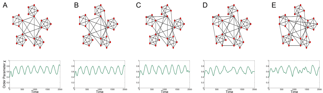
Figure 4. Kuramoto simulations for rewired hierarchical networks. Time series for global order parameter, \chi , for various networks of coupled Kuramoto oscillators. Each network has been rewired using the Xswap rewiring algorithm which maintains the degree of each node. Two pairs of edges have been rewired from one graph to the next from A through to E and that the oscillating behaviour begins to break down as the hierarchical structure is decreased. k=0.2, \sigma(\omega)=0.02 . Again the same initial conditions and internal oscillator frequencies are used as in Figure 2. doi:10.1371/journal.pone.0075569.g004
