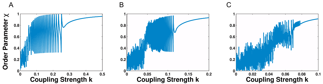
Figure 5. Coupling strength bifurcations for order parameter \chi for networks of clustered random networks Each network contains 3 clusters of 45 randomly connected nodes with approximately 130 connections in each cluster. Here the frequencies are normally distributed with \sigma(\omega) = 0.01 . (A) 50 additional random connections over the whole network; (B) 100 additional connections; (C) 150 additional connections. Note: The oscillatory regions indicate the parameter regimes where oscillatory behaviour will be observed. doi:10.1371/journal.pone.0075569.g005
