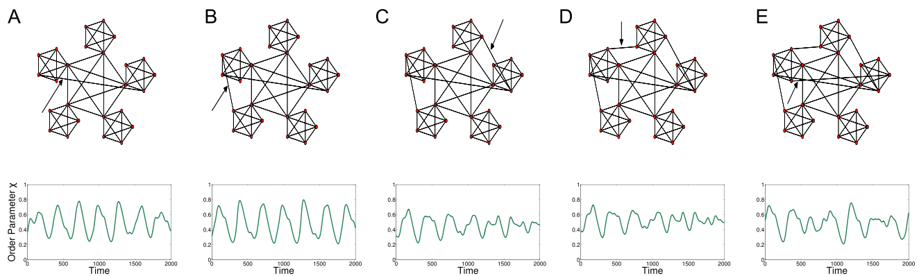
Figure 3. Kuramoto simulation for increasingly perturbed hierarchical network. Time series of global order parameter, \chi , for increasingly perturbed hierarchical network of Kuramoto oscillators. New links are highlighted by arrows, demonstrating the robustness of dynamics to symmetry breaking, with k=0.2, \sigma(\omega)=0.02 . Each simulation uses the same initial conditions and oscillator frequencies as in Figure 2. Similar observations occur whether the simulations are conducted as individual runs (as shown here) or with the network structure being perturbed as the simulation is performed. Note: Although the time series for C and D appear very similar they are simulations from their respective graphs. doi:10.1371/journal.pone.0075569.g003
