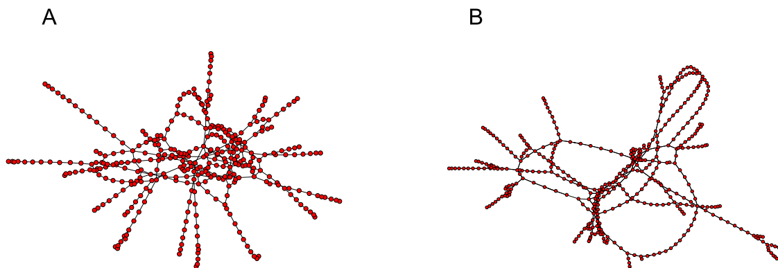
Figure 12. Graphical representations of two underground railway networks. The London Underground (A) and New York Metro (B) networks, represented as non spatially-arranged graphs (i.e. they represent station connectivity, rather than the actual geographical locations of stations). Note the presence of two central clusters in the New York graph, which represent the concentration of stations in South Manhattan and Brooklyn. Both of these networks representations were generated using the Mathematica spring algorithm. doi:10.1371/journal.pone.0075569.g012
