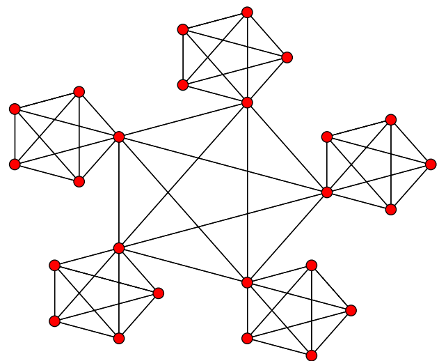
Figure 1. Example graph with community structure (one level of hierarchy). For such a network there exist parameter regimes where the smaller, globally connected sub-graphs may synchronise but the network as a whole does not (partial synchronisation or clustering). doi:10.1371/journal.pone.0075569.g001
