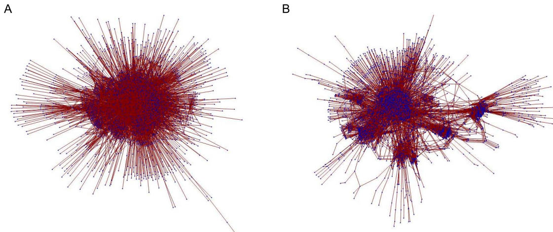
Figure 9. Graphical representations of two versions of the same human metabolic network. (A) Non-partitioned representation of human metabolic network. (B) Partitioned representation of human metabolic network in which the network is partitioned into sub-cellular networks. The Mathematica spring algorithm is used to display the network structures, it is apparent that the two versions have a very different structure. doi:10.1371/journal.pone.0075569.g009
