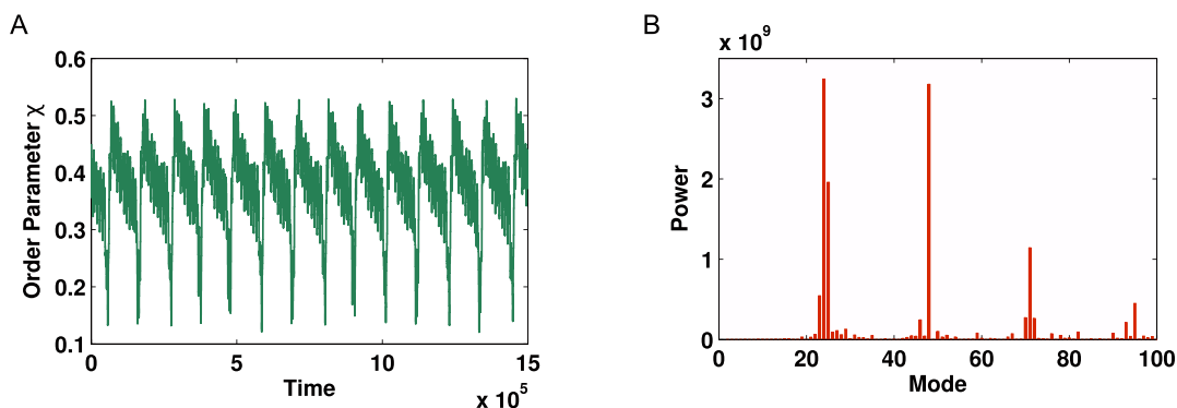
Figure 8. Kuramoto simulation and corresponding Fourier spectrum for the network shown in Figure 7. (A) Time series of global order parameter \chi for a network with two levels of hierarchy with \sigma(\omega)=0.0012 and k=0.12 . (B) Fourier spectrum for the signal in A demonstrating the modes of oscillation in the signal. Two strong peaks can be seen (22 and 46) followed by their respective echoes (66 and 93). doi:10.1371/journal.pone.0075569.g008
