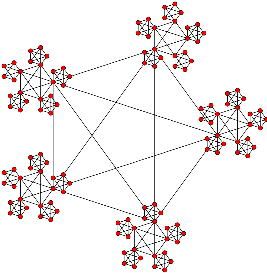
Figure 7. Example graph with community structure (two levels of hierarchy). For such a network there exist parameter regimes where the smaller, globally connected sub-graphs may synchronise but the network as a whole does not (partial synchronisation or clustering). doi:10.1371/journal.pone.0075569.g007
