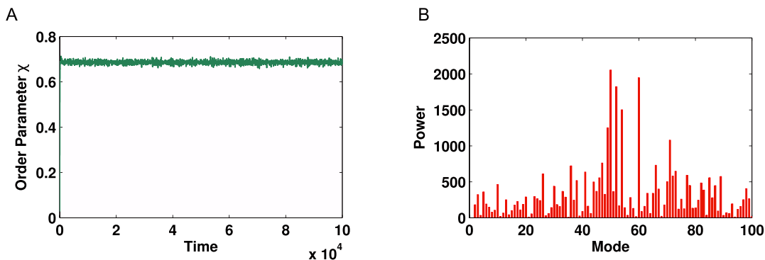
Figure 10. Kuramoto simulation and corresponding Fourier spectrum for the unpartitioned human metabolic network. (A) Time series of global order parameter \chi for the network shown in Figure 9 A with \sigma(\omega)=0.02, k=30.63 . As no region of oscillation was found in the bifurcations for this network, parameter values were set to the same as those for the partitioned network, for the purposes of comparison. (B) Corresponding Fourier spectrum showing no strong peaks due to the signal not showing oscillatory behaviour. doi:10.1371/journal.pone.0075569.g010
