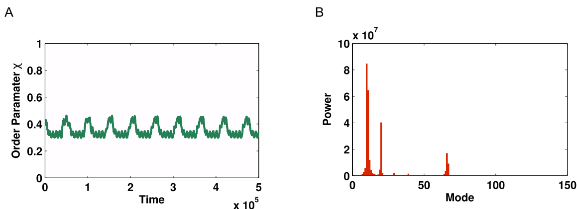
Figure 14. Kuramoto simulation and corresponding Fourier spectrum for the New York Metro. (A) Time series of global order parameter \chi for the network shown in Figure 12 B with \sigma(\omega)=0.0028, k=6.5 . These values were chosen to maximise the oscillatory behaviour. (B) Corresponding Fourier spectrum for signal in A. doi:10.1371/journal.pone.0075569.g014
