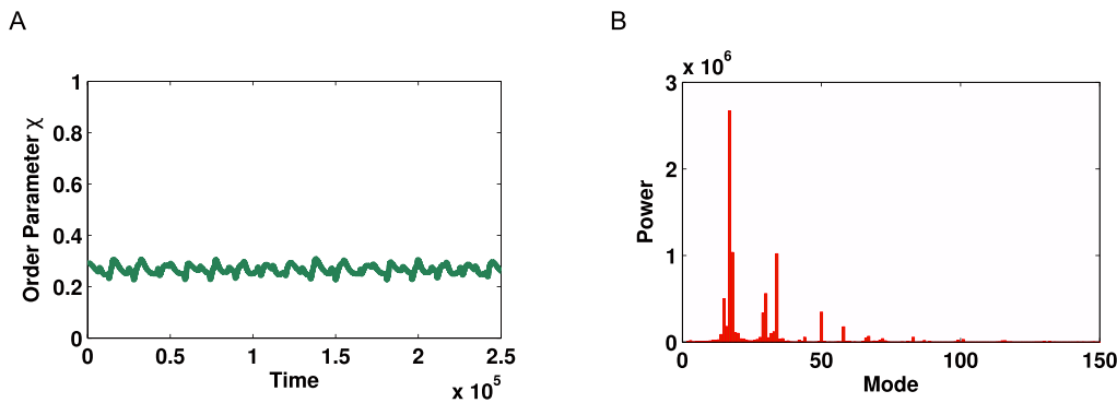
Figure 13. Kuramoto simulation and corresponding Fourier spectrum for the London Underground. (A) Time series of global order parameter \chi for the network shown in Figure 12 A with \sigma(\omega)=0.0021, k=3.6 . These values were chosen to maximise the oscillatory behaviour. (B) Corresponding Fourier spectrum for signal in A . doi:10.1371/journal.pone.0075569.g013
