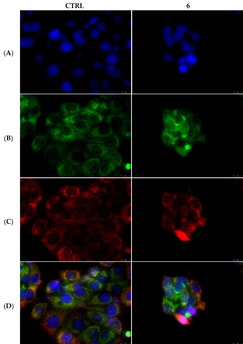
Figure 12. Mitochondria staining and cytochrome c detection in MCF-7 cells. In the CTRL cells as well as in the cells treated with compound 6 at its IC50 value for 24 h, cytochrome c is localized within mitochondria. Panels (A), DAPI \lambda_{\text{ex/em}} = 350/460 nm; Panels (B), Alexa Fluor CF 488 \lambda_{\text{ex/em}} = 490/515 nm; Panels (C), MitoTracker Deep Red FM probe \lambda_{\text{ex/em}} = 644/665 nm; Panels (D), overlay channels. Images were acquired at 40 \times magnification and representative fields are shown.
