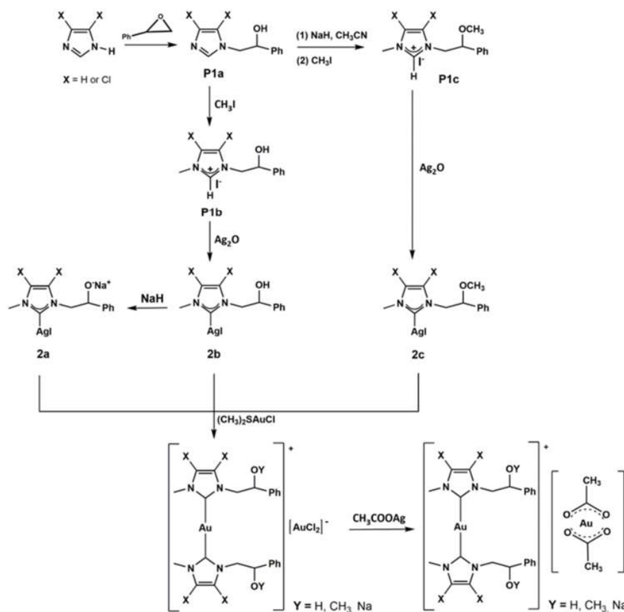
Figure 1. New synthesized Au N-heterocyclic (NHC) carbene complexes.
