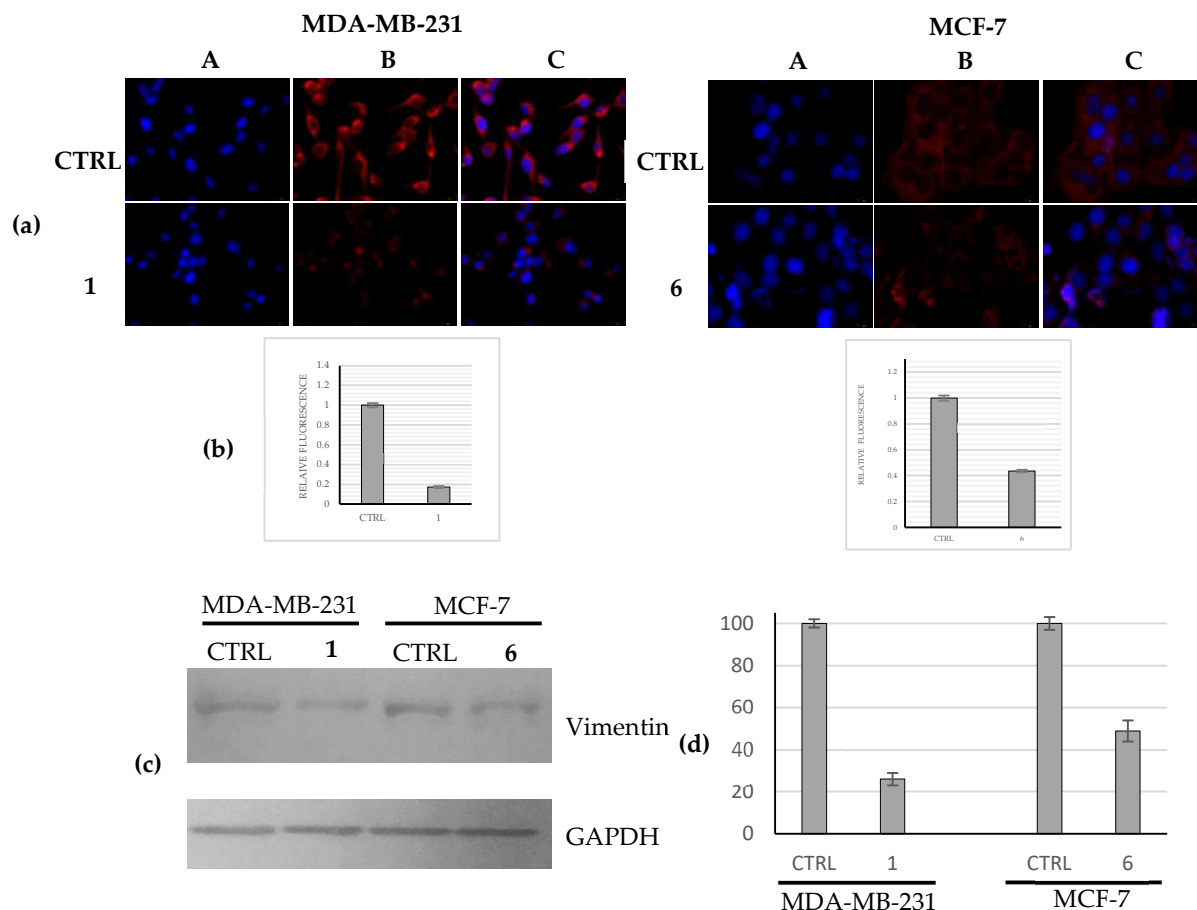
Figure 6. Evaluation of vimentin expression levels. (a) Immunofluorescence studies: MDA-MB-231 and MCF-7 cells were treated with compounds 1 and 6, respectively, (used at their IC_{50} values) or with a vehicle (CTRL) for 24 h. After treatment, the cells were further processed, observed and imaged under the inverted fluorescence microscope at 40\times magnification (for more details see Materials and Methods). Compound 1 induced a downregulation of the vimentin expression with respect to the CTRL cells in MDA-MB-231 cells. Panels A: nuclear stain with DAPI ( \lambda_{ex}/\lambda_{em} = 350/460 nm); Panels B: vimentin (Alexa Fluor ® 568; \lambda_{ex}/\lambda_{em} = 644/665 nm); Panels C: show a merge. Images are representative of three separate experiments; (b) Fluorescence quantification carried out using ImageJ; p < 0.001 ; (c) Western blots analysis: MDA-MB-231 and MCF-7 cells were treated with compounds 1 and 6, respectively, (used at their IC_{50} values) or with a vehicle (CTRL) for 24 h and then the total protein content was extracted and processed as reported in the Experimental Section. GAPDH: loading normalization. Images are representative of three separate experiments; (d) Western blots quantification carried out using ImageJ; p < 0.001 .
