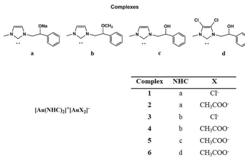
Scheme 1. NHC-Au(I) complexes.
