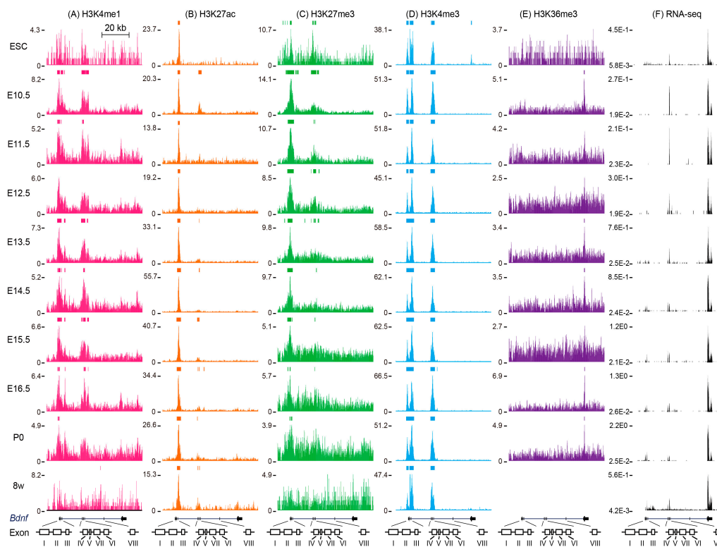
Figure 2. Histone modifications at mouse Bdnf gene during brain development. All data were collected from the ENCODE database and visualized in the University of California Santa Cruz (UCSC) genome browser with the alignment to mouse genome assembly (GRCm38/mm10). The bars located above the peaks indicate the confident enrichments of these histone marks. ESC: embryonic stem cell; E10.5–E16.5: embryonic day 10.5–16.5; P0: postnatal day 0; 8 w: eight weeks adult cerebellum. (A) The accession numbers of H3K4me1 mark are ENCSR000CBF, 272GNQ, 450ITF, 157IVC, 253IEG, 037HLB, 449EUZ, 678FIT, 391WSS and 000CAL (ESC, E10.5–E16.5, P0 and 8 w, respectively). (B) The accession numbers of H3K27ac mark are ENCSR000CDE, 989LUY, 088UKA, 252ONR, 671NSS, 254AHA, 428GHF, 553I WV, 672ZXY and 000CDC (ESC, E10.5–E16.5, P0 and 8 w, respectively). (C) The accession numbers of H3K27me3 mark are ENCSR000CFN, 966TCN, 545BRW, 104PWP, 129OJN, 929GXP, 857GQI, 465TIZ, 340ROY and 000CFN (ESC, E10.5–E16.5, P0 and 8 w, respectively). (D) The accession numbers of H3K4me3 mark are ENCSR000CBG, 581EJK, 283RFW, 554TSO, 167ZGV, 203KIB, 486MHP, 637CCT, 427ZJU and 000CAK (ESC, E10.5–E16.5, P0 and 8 w, respectively). (E) The accession numbers of H3K36me3 mark are ENCSR000CFO, 747ZXL, 535NVE, 764UIE, 066WUD, 702JYV, 487RAU, 205XBQ and 951UWY (ESC, E10.5–E16.5 and P0, respectively). (F) The accession numbers of RNA-seq are ENCSR000CWC, 764OPZ, 307BCA, 908JWT, 792RJV, 343YLB, 557RMA, 367ZPZ, 255SDF and 000BZM (ESC, E10.5–E16.5, P0 and 8 w, respectively).
