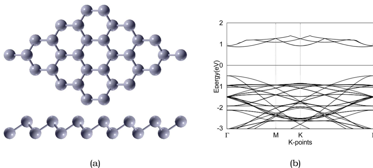
Fig. 3 Atomic structure and band structure of 4 \times 4 \times 1 pristine antimonene. The Fermi level is set to 0. Sb is represented by silver, respectively.
